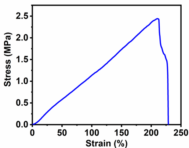
Figure S1. Tensile stress-strain curve of the bioinspired dressing.
