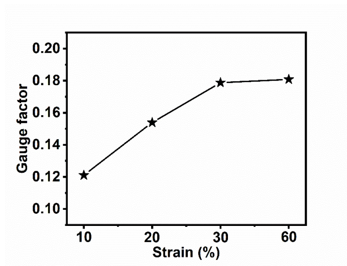
Figure S3. The gauge factors of dressing in different tensile strains.
