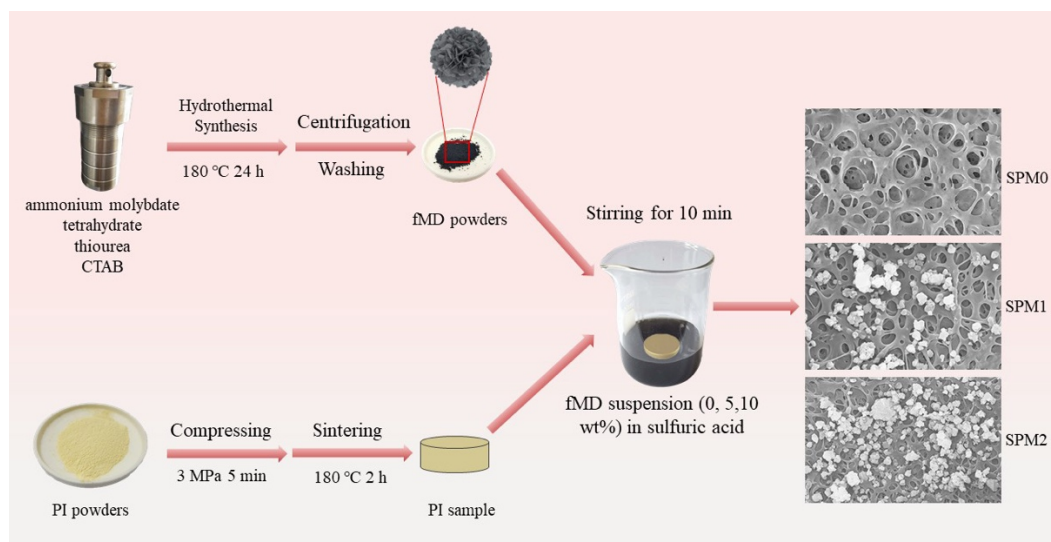
Fig. S1 Schematic illustration of synthesis of fMD and fabrication of SPM0, SPM1 and SPM2
