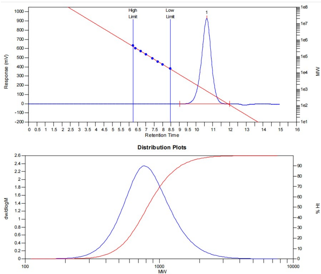
Supplementary Figure 2. The GPC profile of inulin. The mobile phase was H 2 O with a flow rate of 1.0 mL/min.
