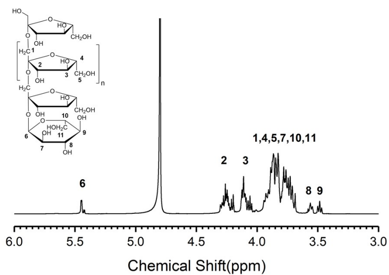
Supplementary Figure 1. ^1\text{H} NMR spectrum of inulin in \text{D}_2\text{O} .
