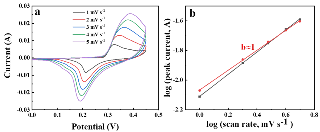
Fig.S2. (a) CV curves at 1-5 mV s -1 of Co-NTC@Co 3 S 4 , (b) linear fitting diagram of log I and log v .
