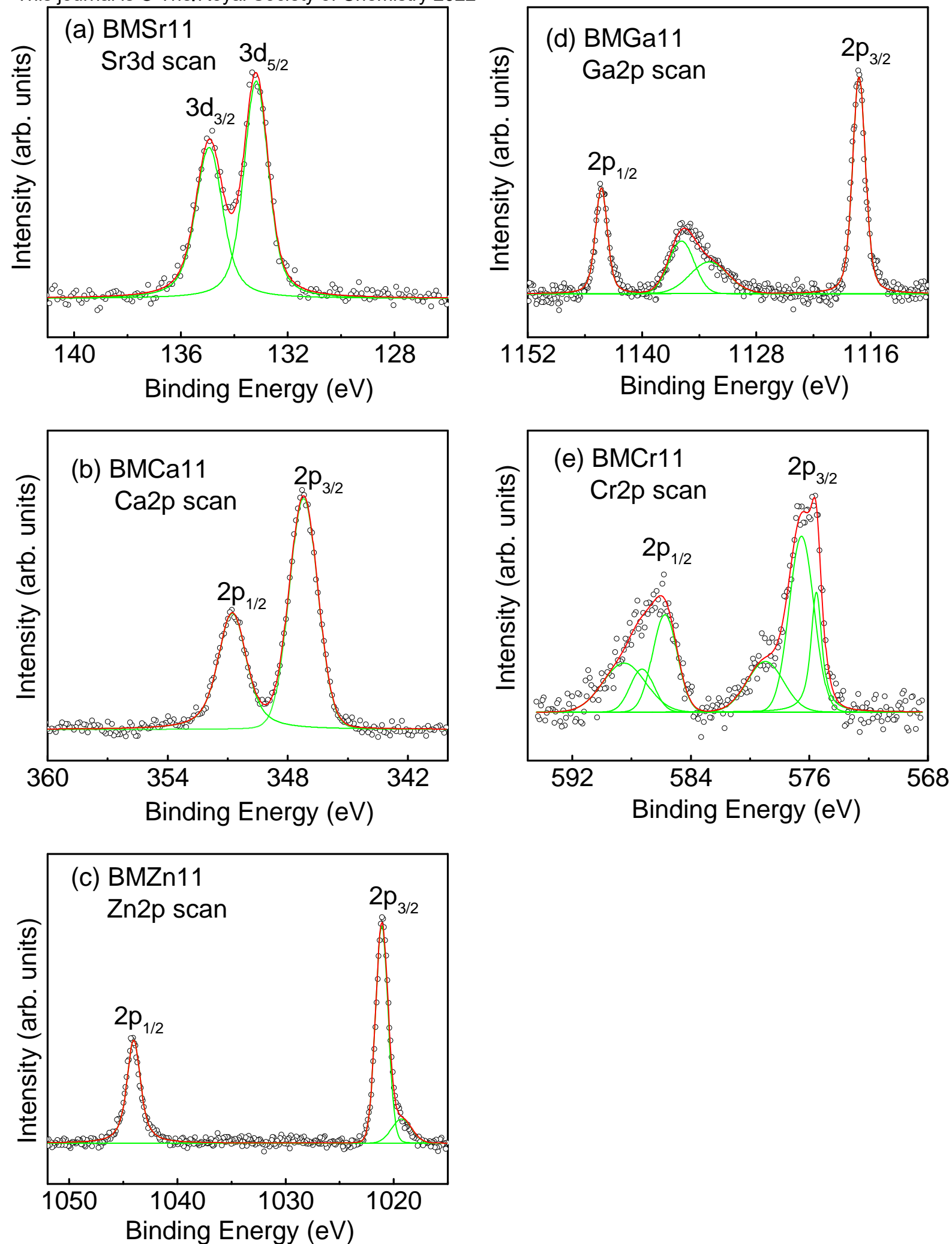
Fig. S2. XPS plots of dopants scan of Ba-site doping (a-c) and Fe-site doping (d-e) of samples heated at 1100 °C.
