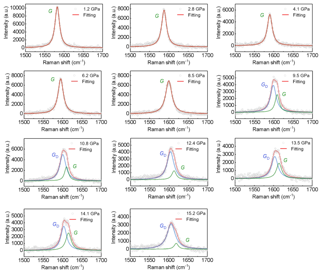
Figure S1. The Raman spectrum of HOPG at different pressures from 1.2 GPa to 15.2 GPa with MEW as PTM. The solid lines are Lorentzian fit to the experimental data.
