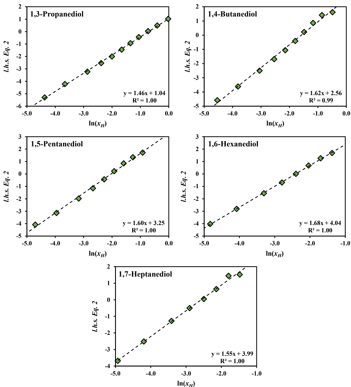
Figure S3. Left-hand-side of Equation 2 as a function of the natural logarithm of hydrotrope mole fraction in the water/hydrotrope/solute ternary mixture for syringic acid and the 1, n -alkanediols studied in this work at (303.2 ± 0.5) K. Dashed lines represent the best linear fitting obtained using the method of least squares. The slope and intercept of the linear fitting correspond to parameters m and b of the cooperative model of hydrotrophy.
