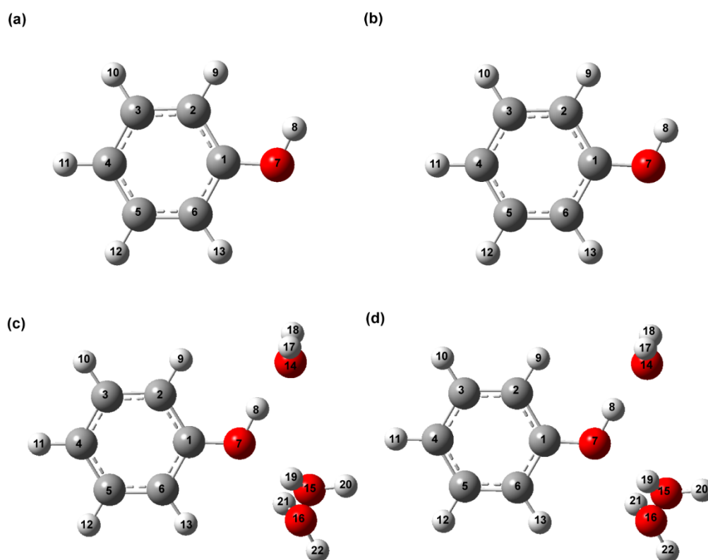
Fig. S10. The equilibrium geometries of the (a) phenol radical cation, (b) deuterated phenol radical cation, (c) microhydrated phenol radical cation, \text{PhOH}\cdot^+(\text{H}_2\text{O})_3 , and (d) microhydrated deuterated phenol radical cation, \text{PhOD}\cdot^+(\text{D}_2\text{O})_3 , in aqueous solution. The carbon, oxygen and hydrogen atoms are in gray, red and white respectively.
