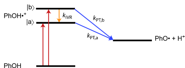
Fig. S8. Schematic energy level diagram of phenol (PhOH), phenol radical cation (PhOH •+ ) and phenoxy radical (PhO • ). States |a\rangle and |b\rangle correspond to the vibrational ground and excited states of the vibrational modes of phenol radical cation with dominant OH or OD character. These vibrational states can undergo depopulation via proton transfer (PT), while the vibrationally excited state can also undergo intramolecular vibrational relaxation (IVR).
