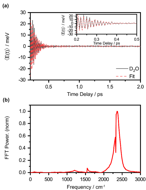
Fig. S6. (a) First-moment time trace, \langle E(t) \rangle , of the ionized liquid D 2 O. The inset shows the enlarged \langle E(t) \rangle from 0.2 ps to 0.5 ps. (b) FFT power spectrum of the first-moment time trace of ionized liquid D 2 O. Note that the O 2 and N 2 vibrational frequencies are also observed at 1552 \text{ cm}^{-1} and 2334 \text{ cm}^{-1} , respectively.
