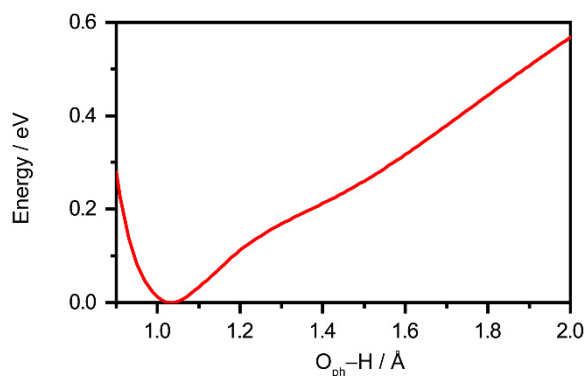
Fig. S9. Potential energy curve as a function of the phenol O_{\text{ph}}\text{-H} bond length for the microhydrated phenol radical cation, \text{PhOH}\cdot^+(\text{H}_2\text{O})_3 .
