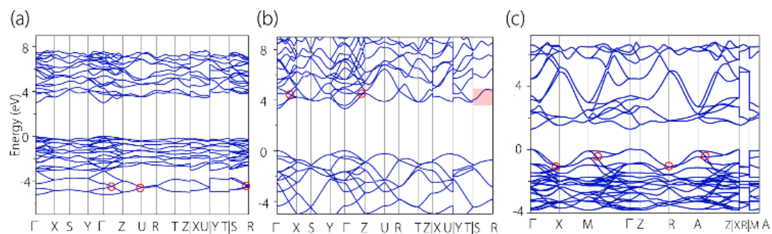
FIG. S1 (a)-(c) The band structures for \text{LiAlSe}_2 , \text{NaMgH}_3 and \text{AuBr} , respectively. SOC is not taken into consideration. The crossing points are highlighted by red circles. The DNL along the S-R path in (b) is shown with red background.
