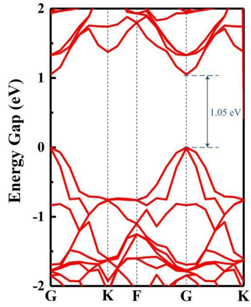
Figure S2. Calculated band structure of Sb/InS bilayer by the HSE06 functional.
