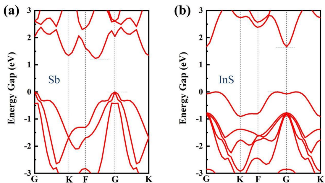
Figure S1. Calculated band structures of (a) Sb and (b) InS monolayer, respectively.
