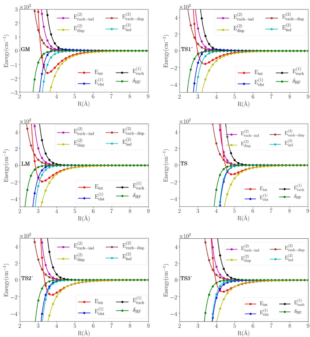
Figure S1: The SAPT/aug-cc-pVTZ contributions are plotted for radial cuts through the 4D-PES passing through each of the 6 structures given in Figure 1.
