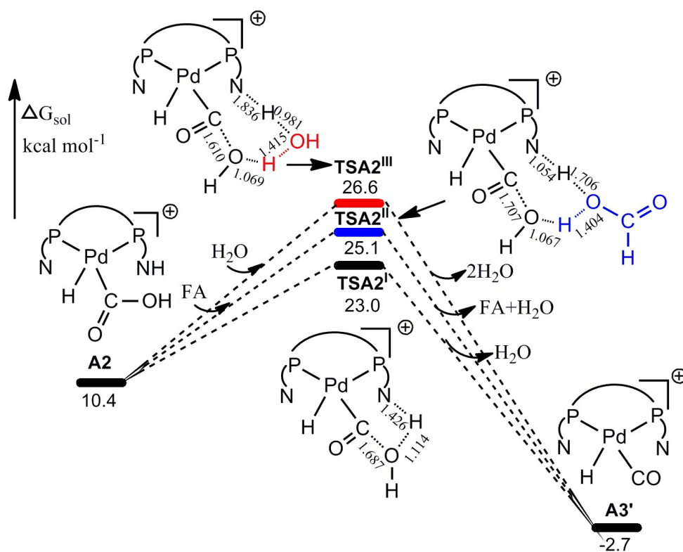
Fig. S1 Calculated free energy profiles with schematic structures for the CO-generation along the NH-Pd pathway.
