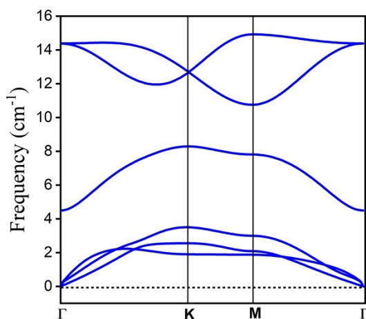
Fig. S1. Phonon spectrum of Bi-C monolayer.
