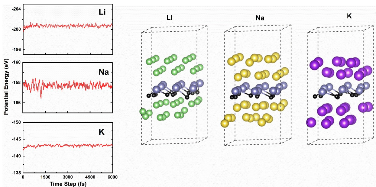
Fig. S2. The ab-initio molecular dynamics calculations of Bi-C monolayer with highest capacity of adatoms at 300 K.
