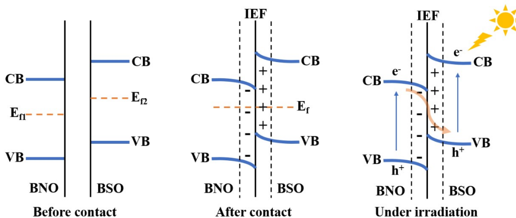
Fig.S2. Schematic diagram of charge transfer path at the BNO/BSO interface
