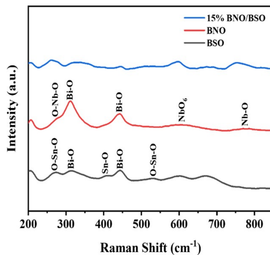
Fig.S1. Raman spectra of pure BNO, BSO and 15%BNO/BSO samples
