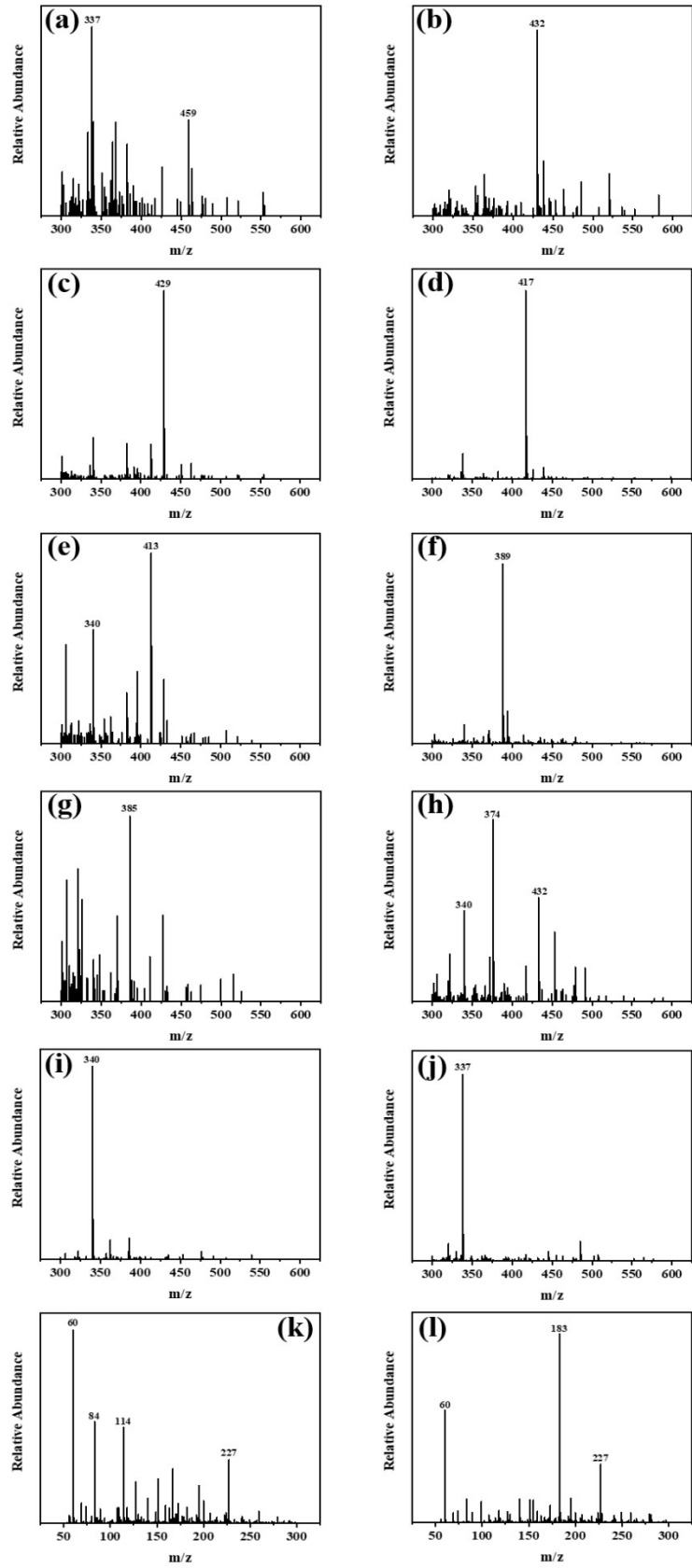
Fig.S3. Mass spectrum of the system when TC was degraded for 60min
