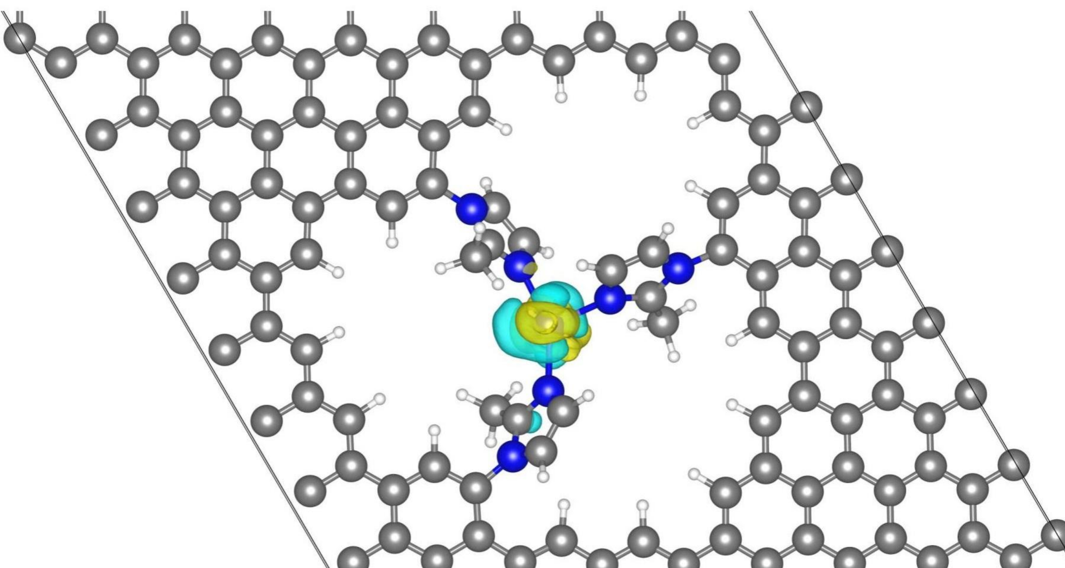
(c) Fe-(mIM) 3
