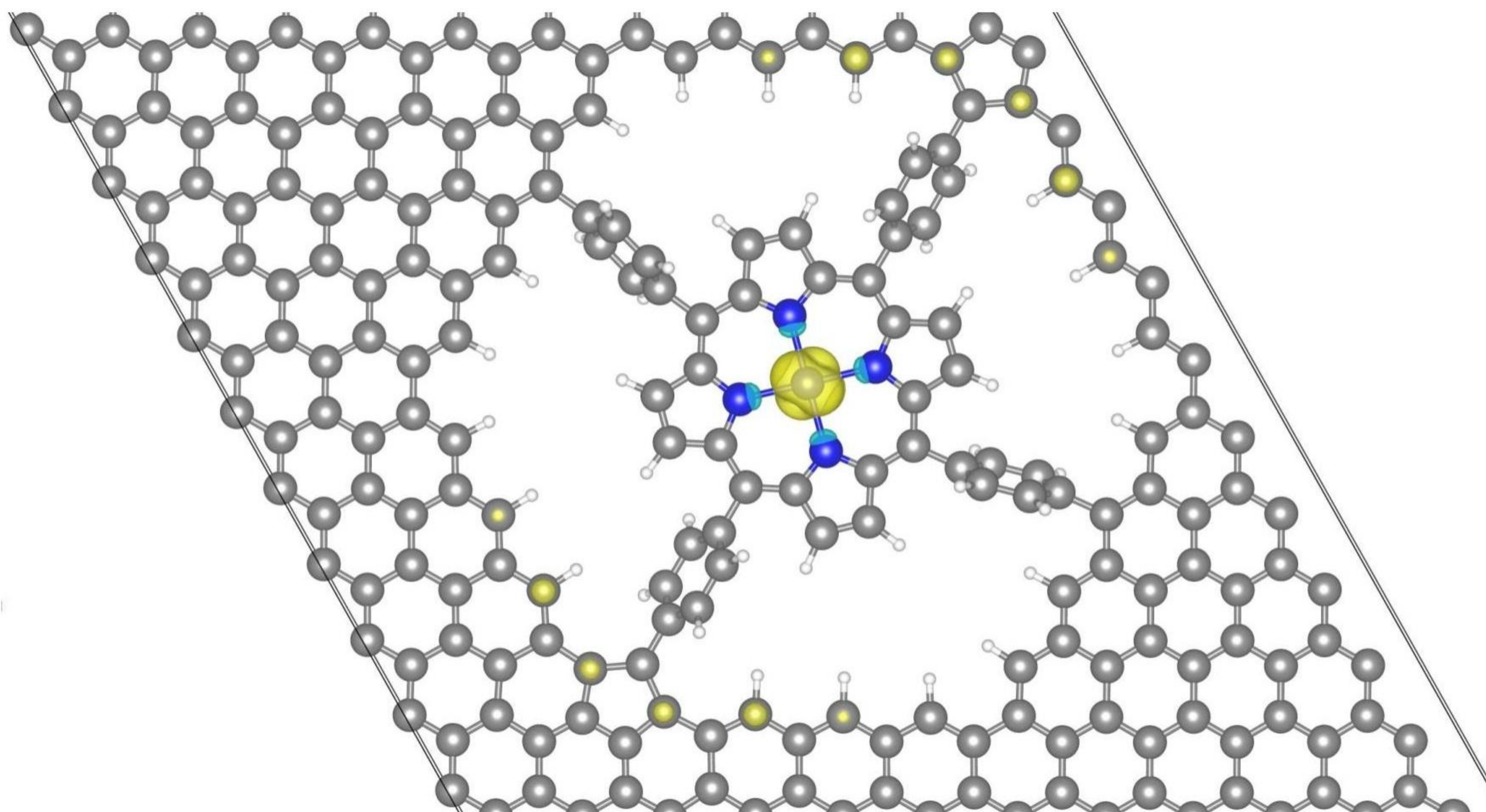
(a) Fe-TCPP
