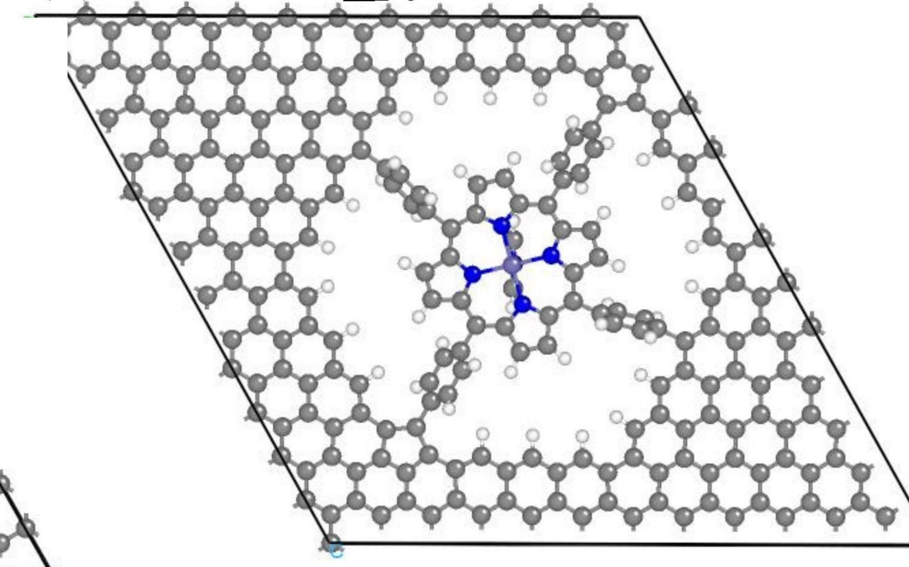
(b) Fe-TCPP_pya
