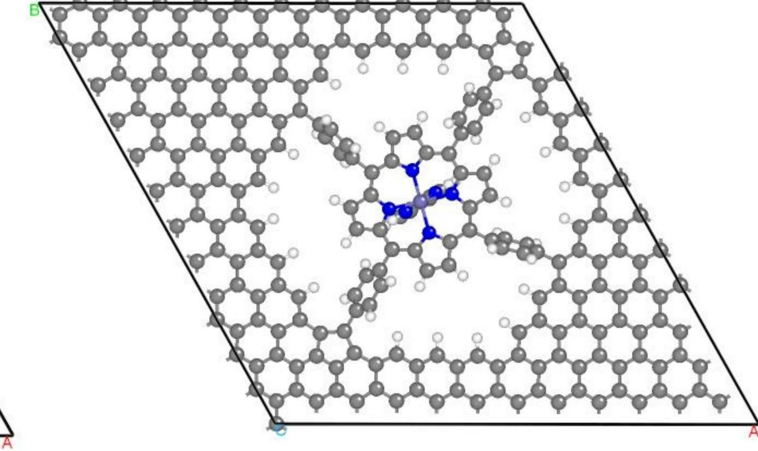
(e) Fe-TCPP_bIm_C
