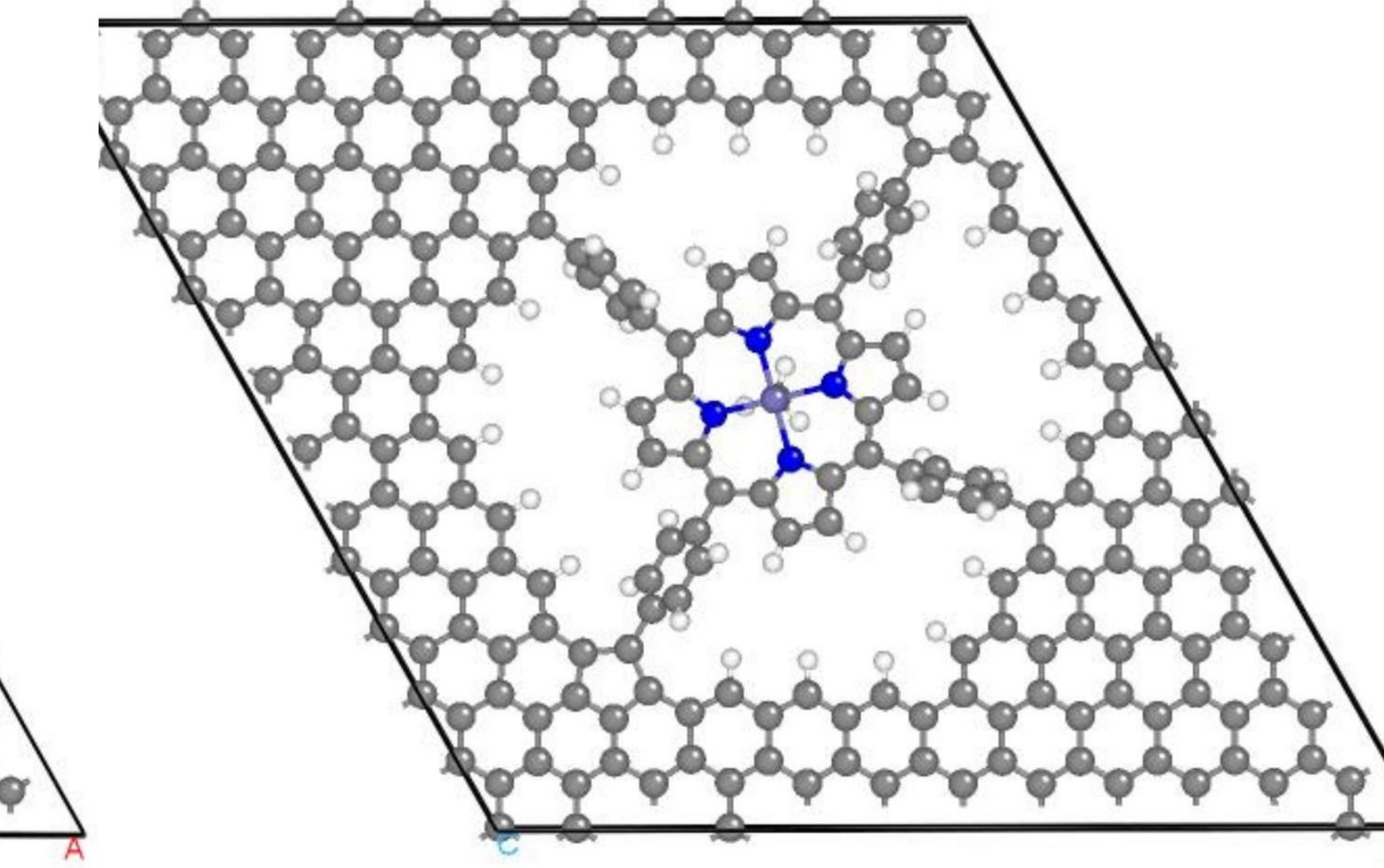
(c) Fe-TCPP_CH 3
