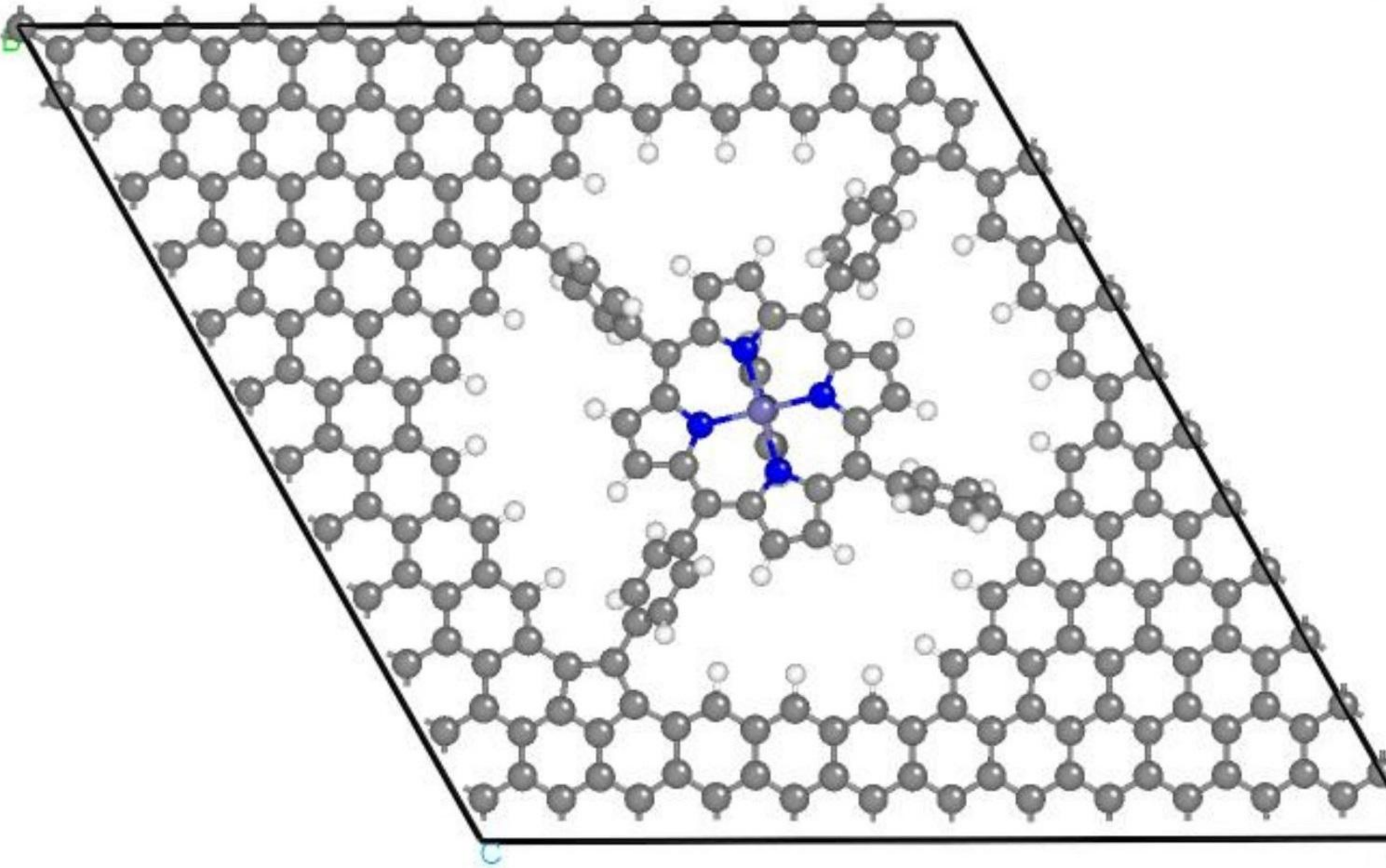
(a) Fe-TCPP_bpy
