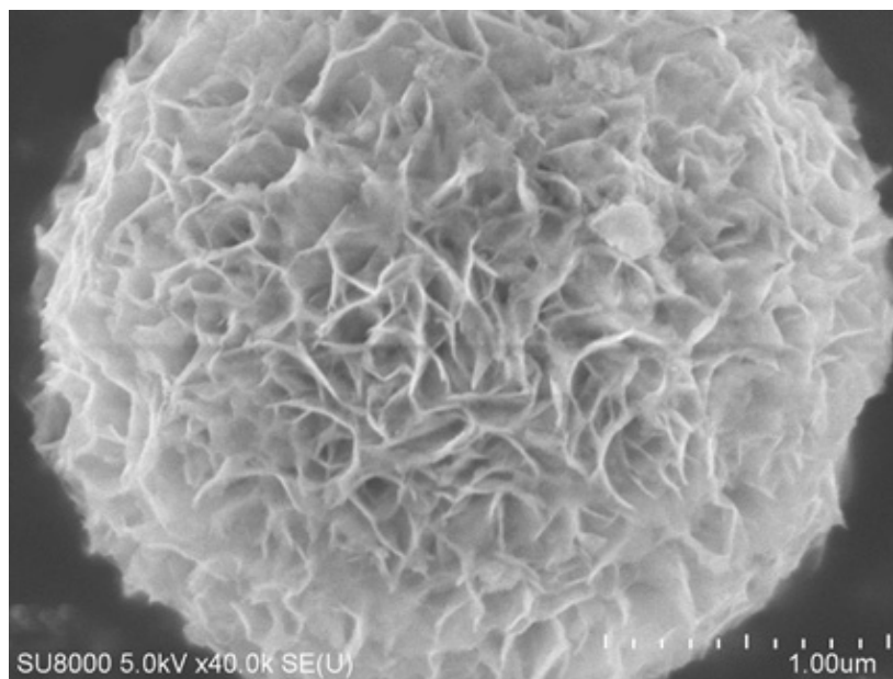
Fig. S1 The SEM image of \text{ZnIn}_2\text{S}_4 .
