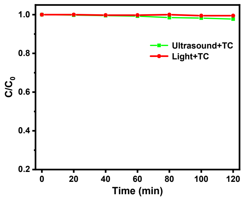
Figure S3. TC degradation curve without photocatalyst under ultrasound and dark (Green), and TC degradation curve without photocatalyst under light irradiation (Red).
