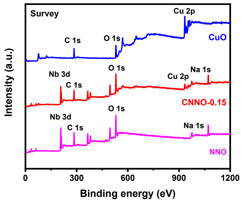
Figure S1. XPS spectra of CuO, NNO, and CNNO-0.15 (survey).
