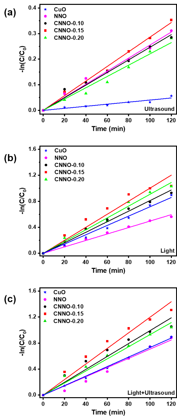
Figure S2. The curves of the TC degradation rate constants under different conditions:
