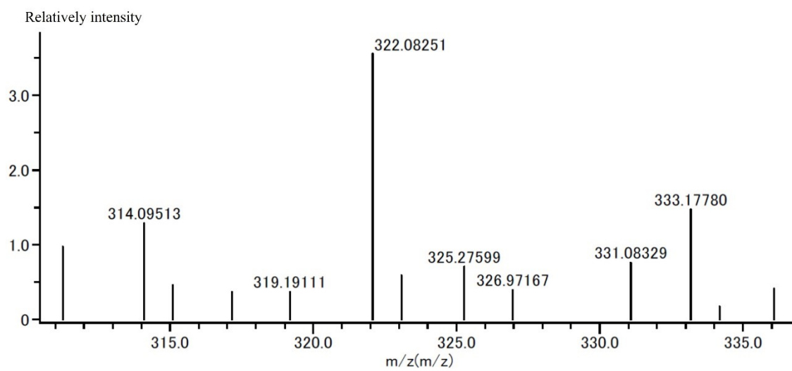
Fig. S3. HRMS spectrum of \text{H}_2\text{L} .
