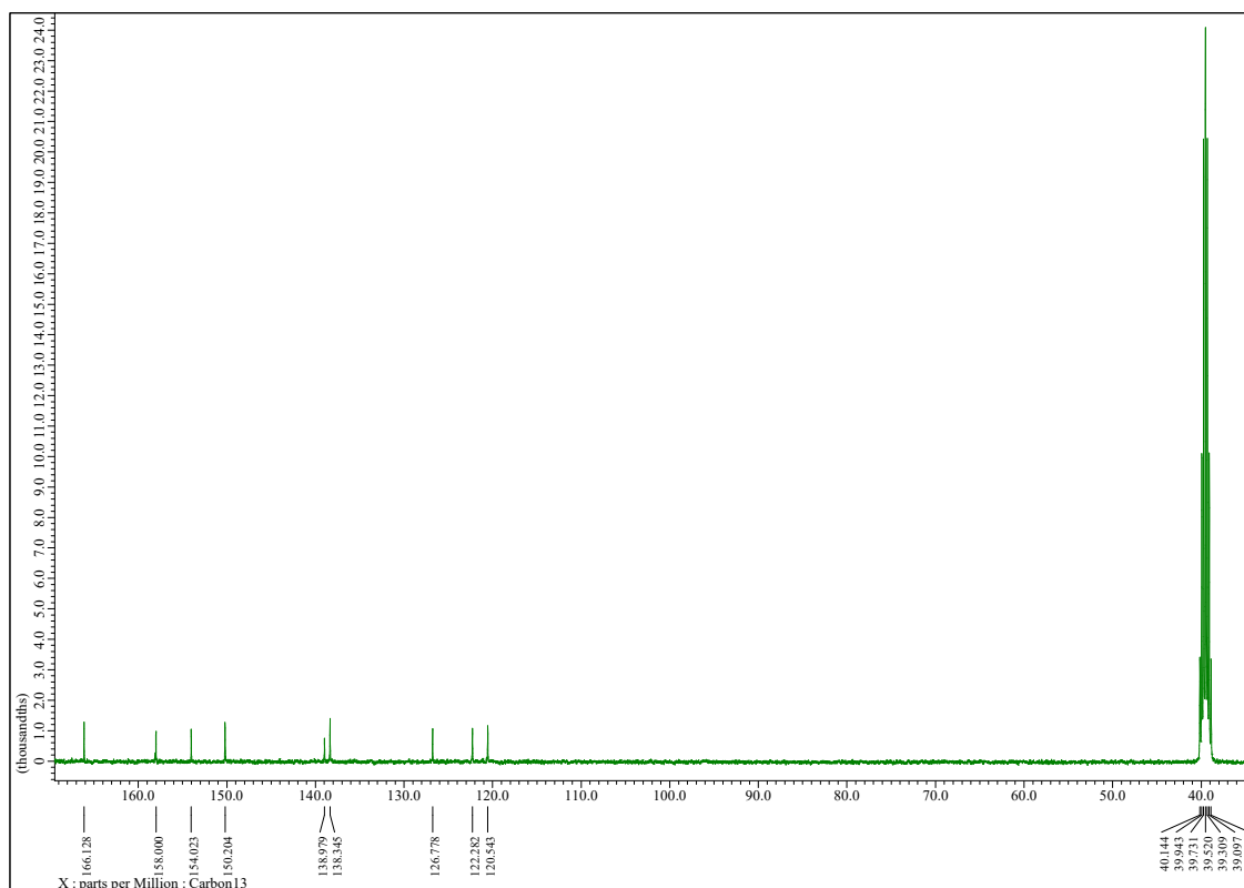
Fig. S1. 1 H NMR spectrum of H 2 L.
