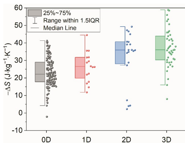
Fig.S1. Magnetic entropy change ( \mu_0\Delta H = 7 T) for the conventional MCE in molecular magnets of different structural dimensionality.
