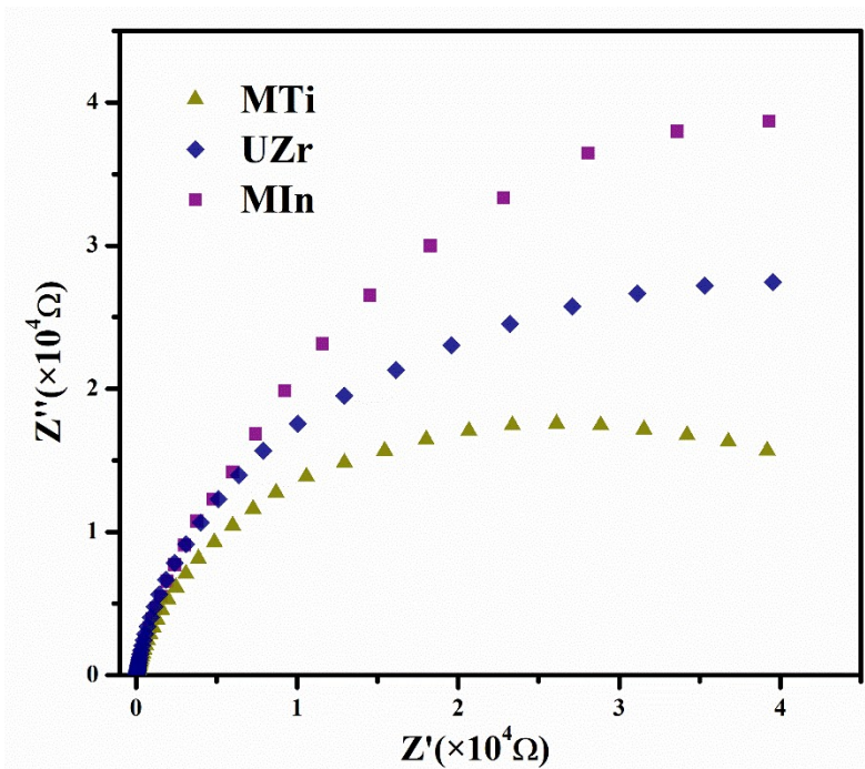
Fig. S3. EIS spectra of as-prepared catalysts.
