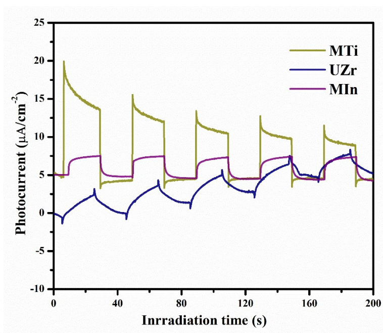
Fig. S4. Transient photocurrent response of as-prepared catalysts.
