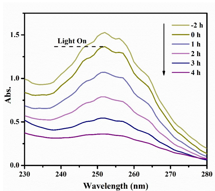
Fig. S2. (b) Time-dependent absorption curves of pyridine/octane solutions over MTi.
