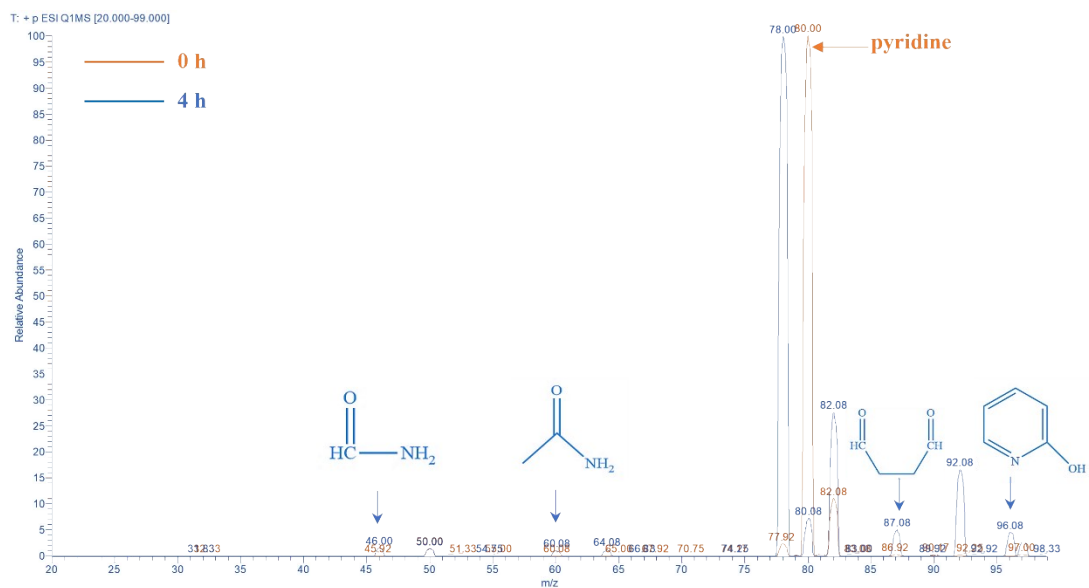
Fig. S5. HPLC-MS spectrogram of denitrification over MTi at different reaction times.
