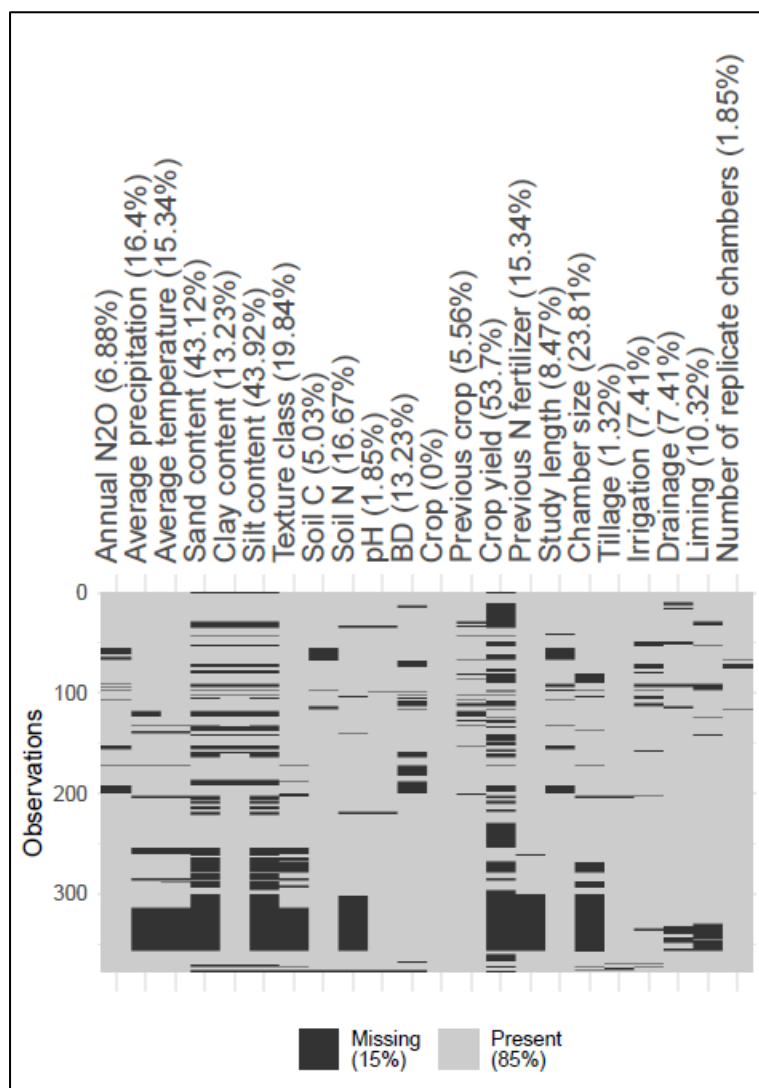
Fig. S1: Missing data pattern in the study
