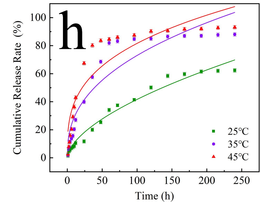
Ritger-Peppas model
