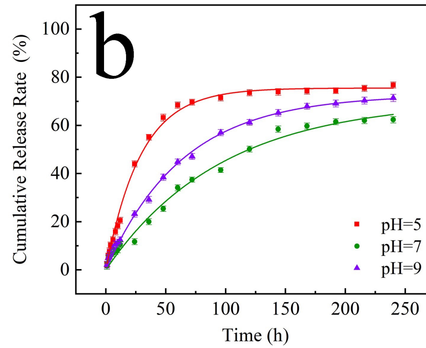
First-order model
