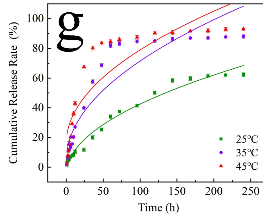
Higuchi model
