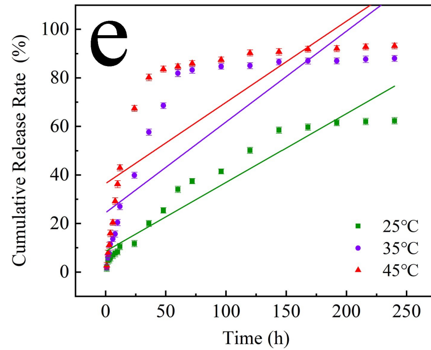
Zero-order model
