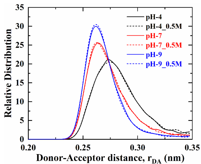
Figure S2. Donor-Acceptor distance for h-bonds formed at the geometric interface of PS-Slab
