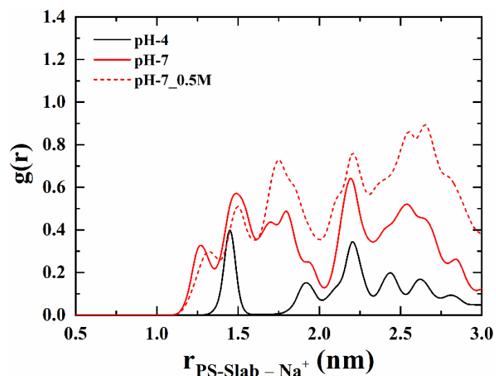
Figure S1. Radial number density distribution of \text{Na}^+ ions at the geometric interface of PS-Slab
