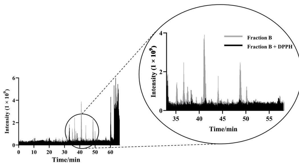
Figure S1. The total ion chromatogram of mass spectrometry.
