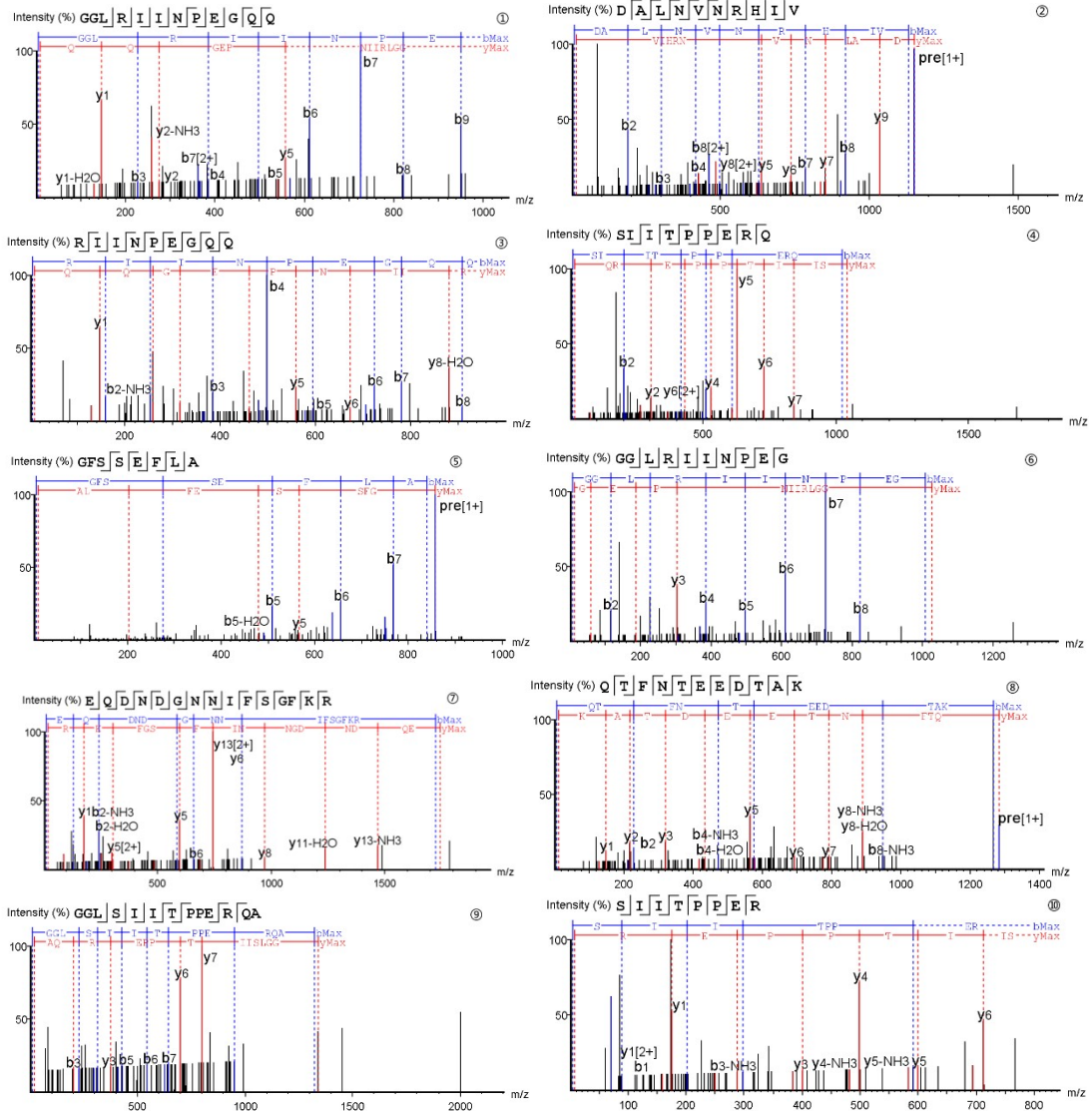
Supplementary Fig. 3. Secondary spectrum of bitter candidate peptides in B-3
