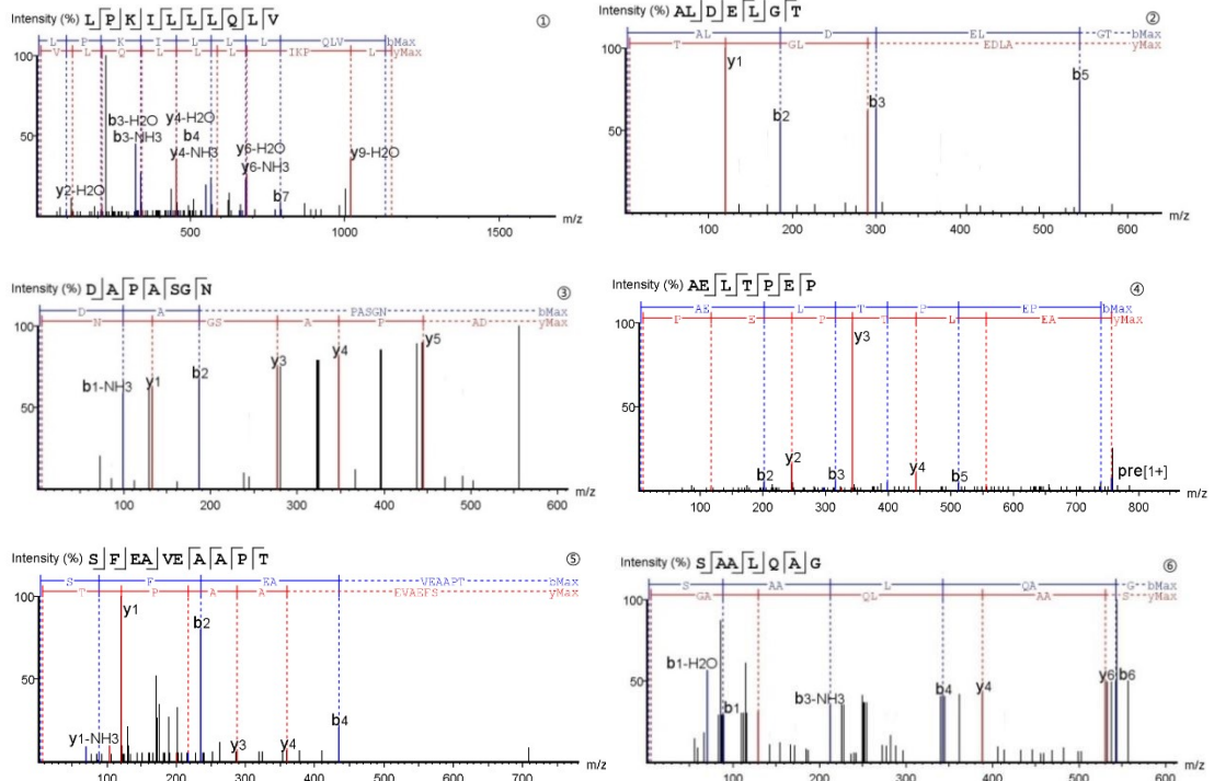
Supplementary Fig. 2. Secondary spectrum of umami candidate peptides in U-2
