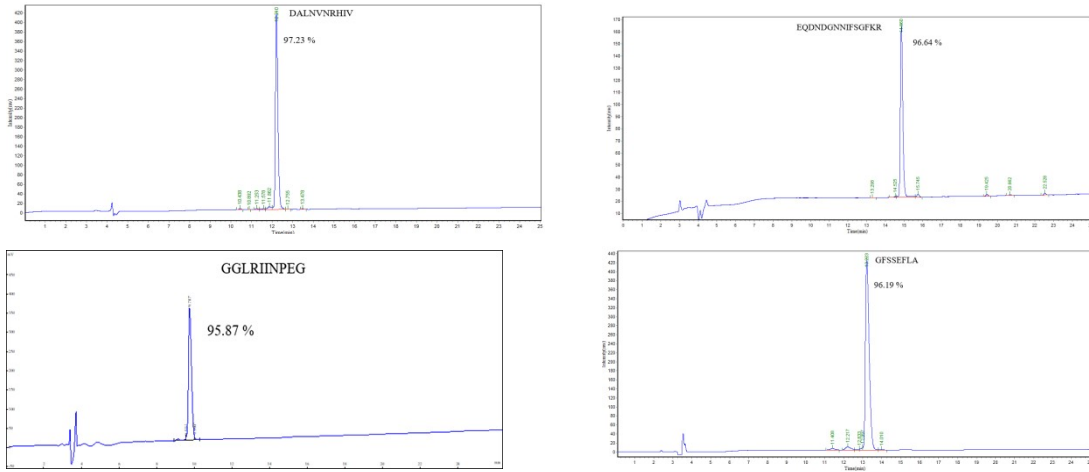
Supplementary Fig. 1. HPLC purity diagram of synthetic peptides
