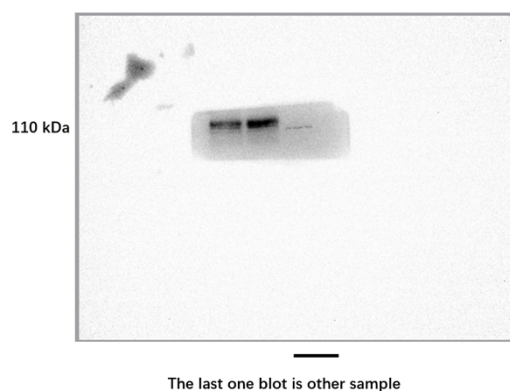
Fig 6A NLRP3
