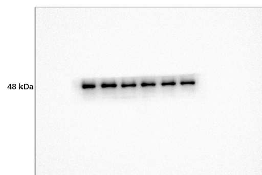
Fig 6B Pro-Caspase-1
