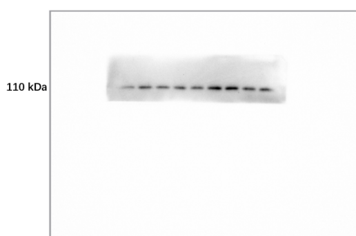
Fig 5B NLRP3
