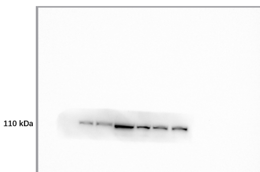
Fig 5D NLRP3
