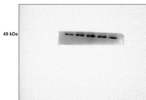
Fig 5K Pro-Caspase-1
