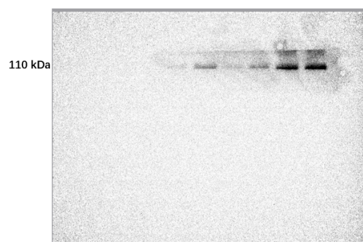
Fig 6B NLRP3
