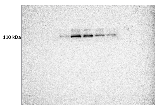
Fig 5K NLRP3
