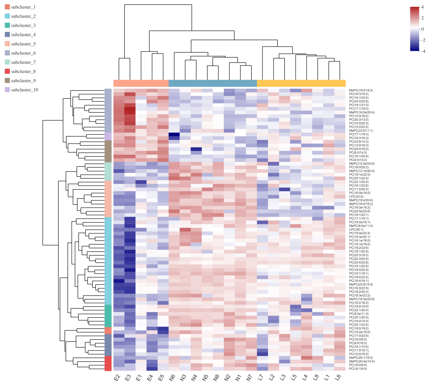
HeatmapTree
