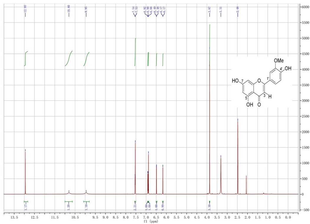
Fig. S6. ^1\text{H-NMR} (600 MHz, \text{DMSO-d}_6 ) and ^{13}\text{C-NMR} (151 MHz, \text{DMSO-d}_6 ) spectrum for Chrysoeriol .
