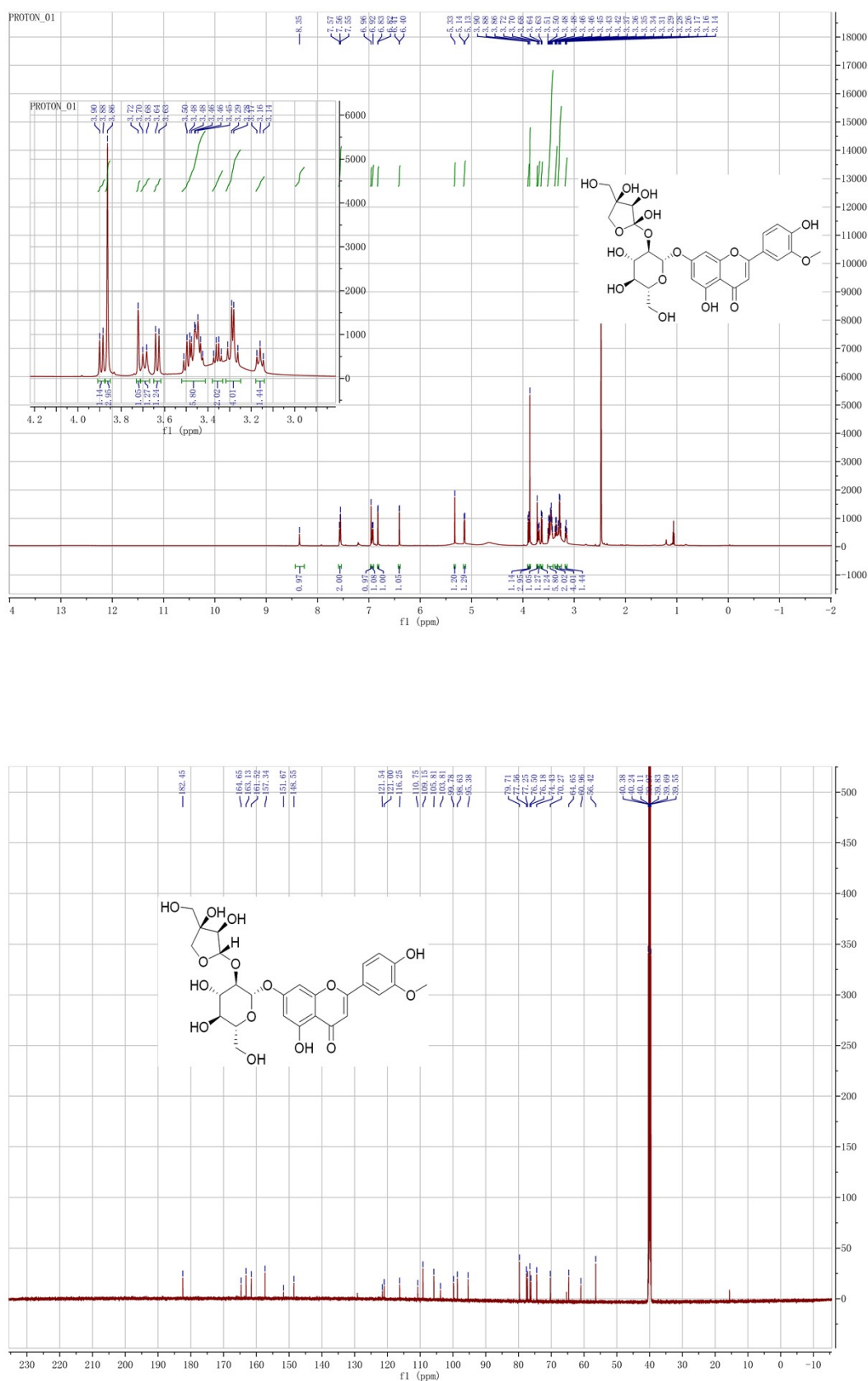
Fig. S5. ^1\text{H-NMR} (600 MHz, \text{DMSO-d}_6 ) and ^{13}\text{C-NMR} (151 MHz, \text{DMSO-d}_6 ) spectrum for Graveobioside B .
