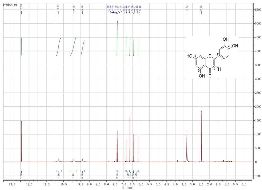
Fig. S4. ^1\text{H} -NMR (600 MHz, DMSO- d_6 ) and ^{13}\text{C} -NMR (151 MHz, DMSO- d_6 ) spectrum for Luteolin .
