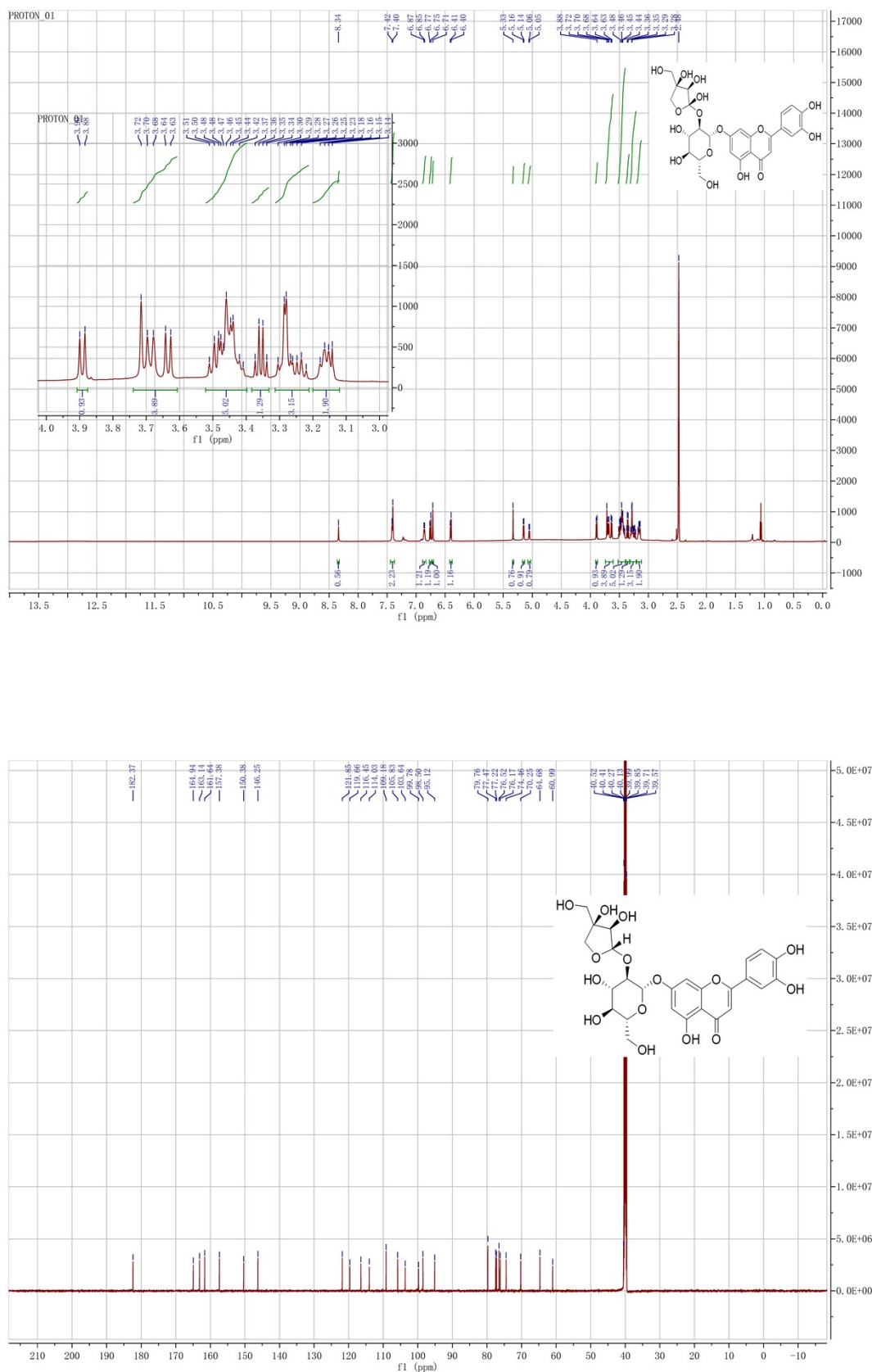
Fig. S3. ^1\text{H-NMR} (600 MHz, \text{DMSO-d}_6 ) and ^{13}\text{C-NMR} (151 MHz, \text{DMSO-d}_6 ) spectrum for Graveobioside A .
