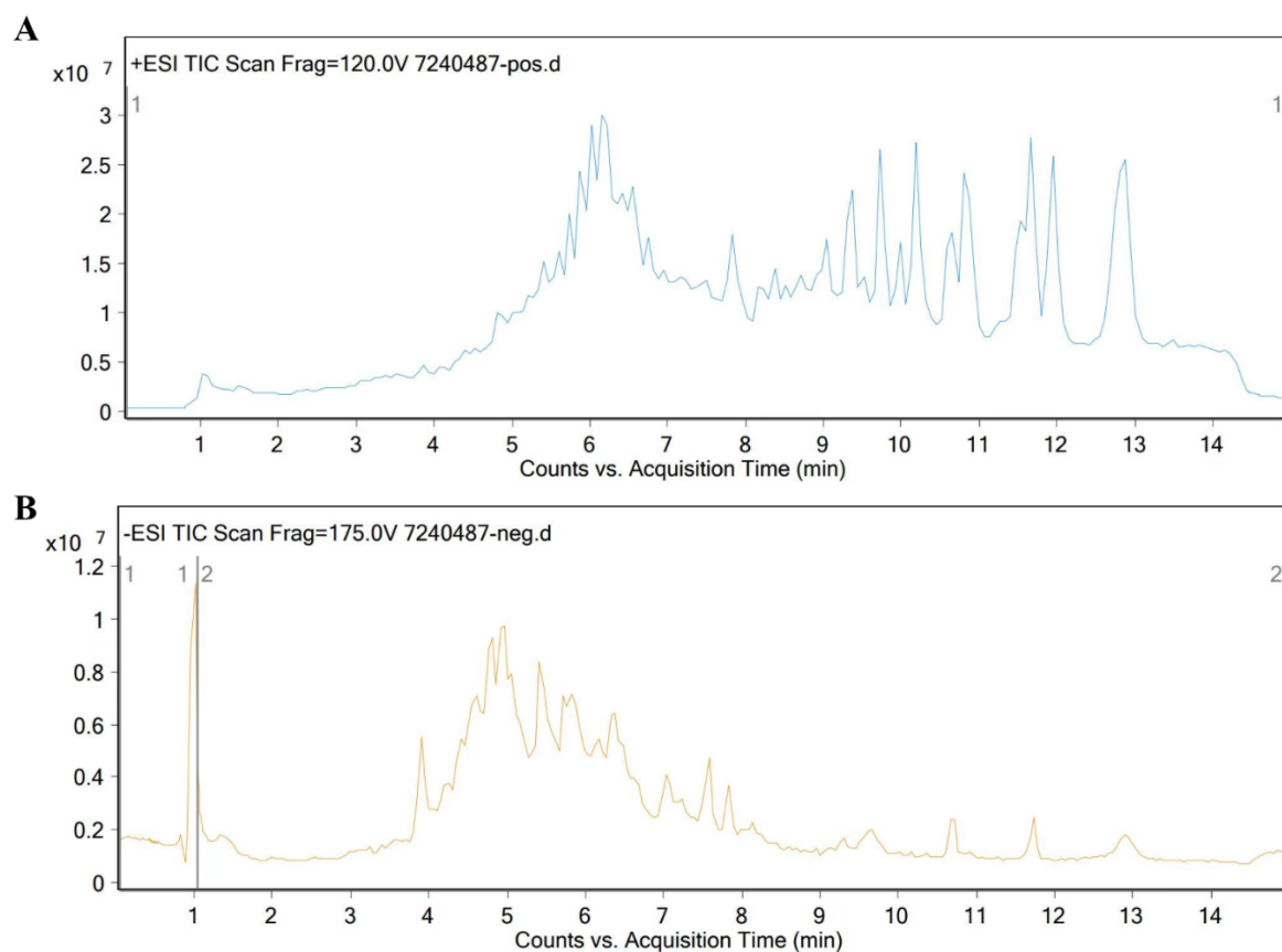
Figure S1. Diagram of LC-MS composition analysis of hawthorn flavonoids. Positive ion chromatogram of hawthorn flavonoid (A), negative anion chromatogram of hawthorn flavonoid (B).
