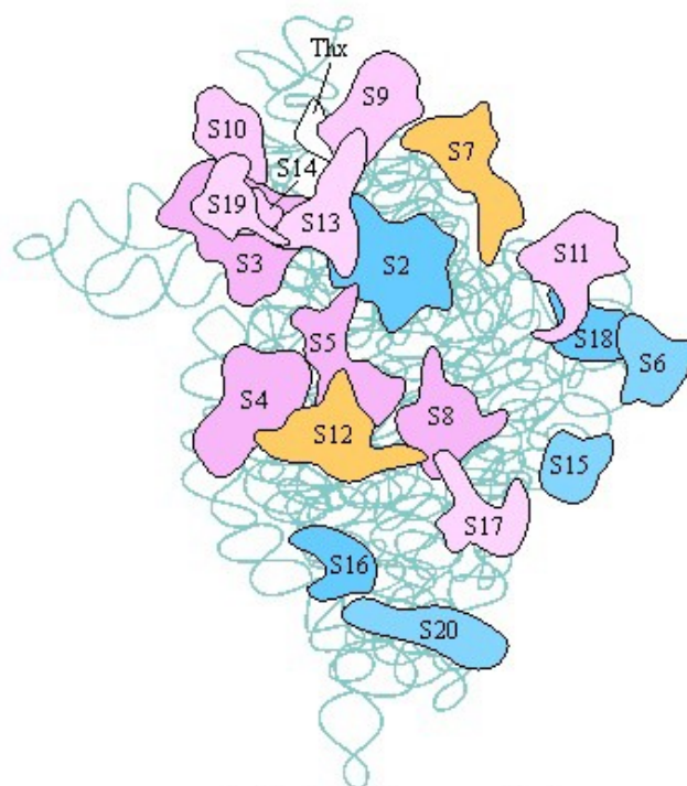
Small subunit ( Thermus aquaticus )
