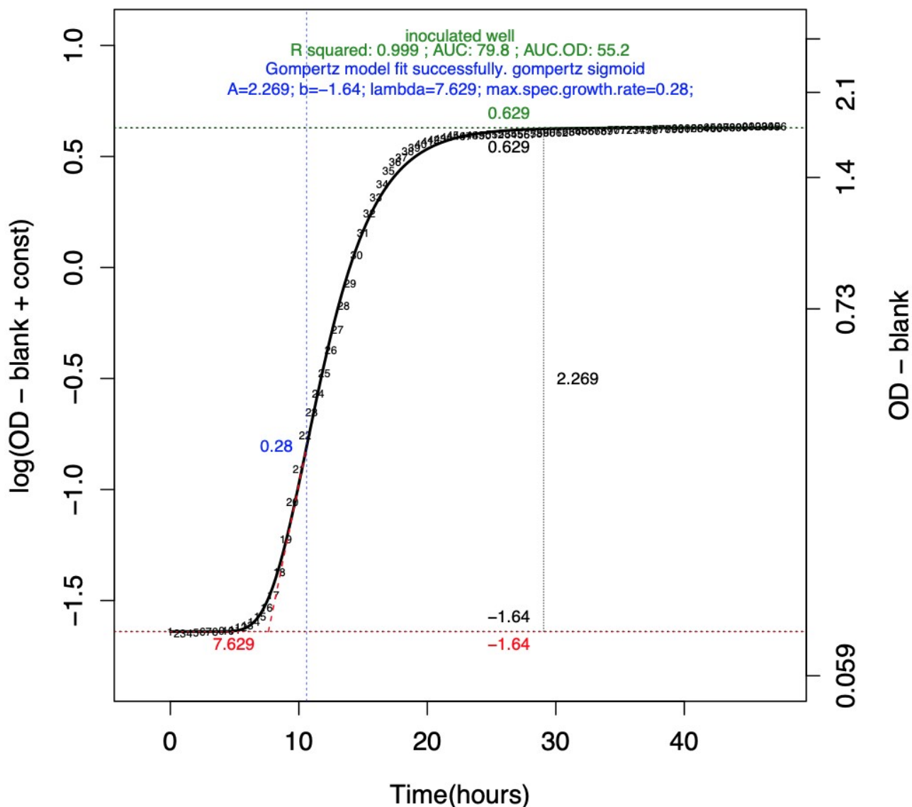
Fig S1: Output of the GCAT fitting of the turbidimetric growth curve (one replicate as example) of L. acidophilus pre-adapted in SUB1 condition and challenged in MRS containing 0.7M sucrose. R squared is the coefficient of determination; AUC is "Area Under the Curve" and AUC.OD is log-transformed AUC.
