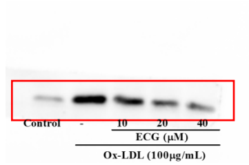
p-I \kappa B \alpha
