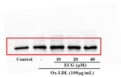
I \kappa B \alpha
