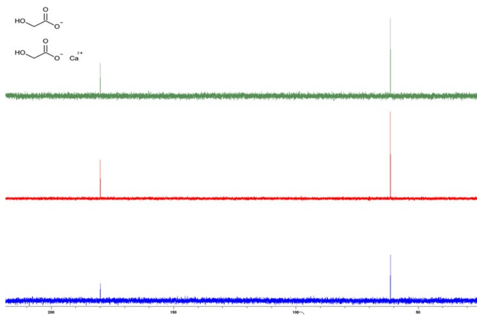
Fig. 1: The NMR spectra of the standard sample (green), 4 th recrystallization CG (red), and 3 rd recrystallization CG (blue) are shown from top to bottom.
