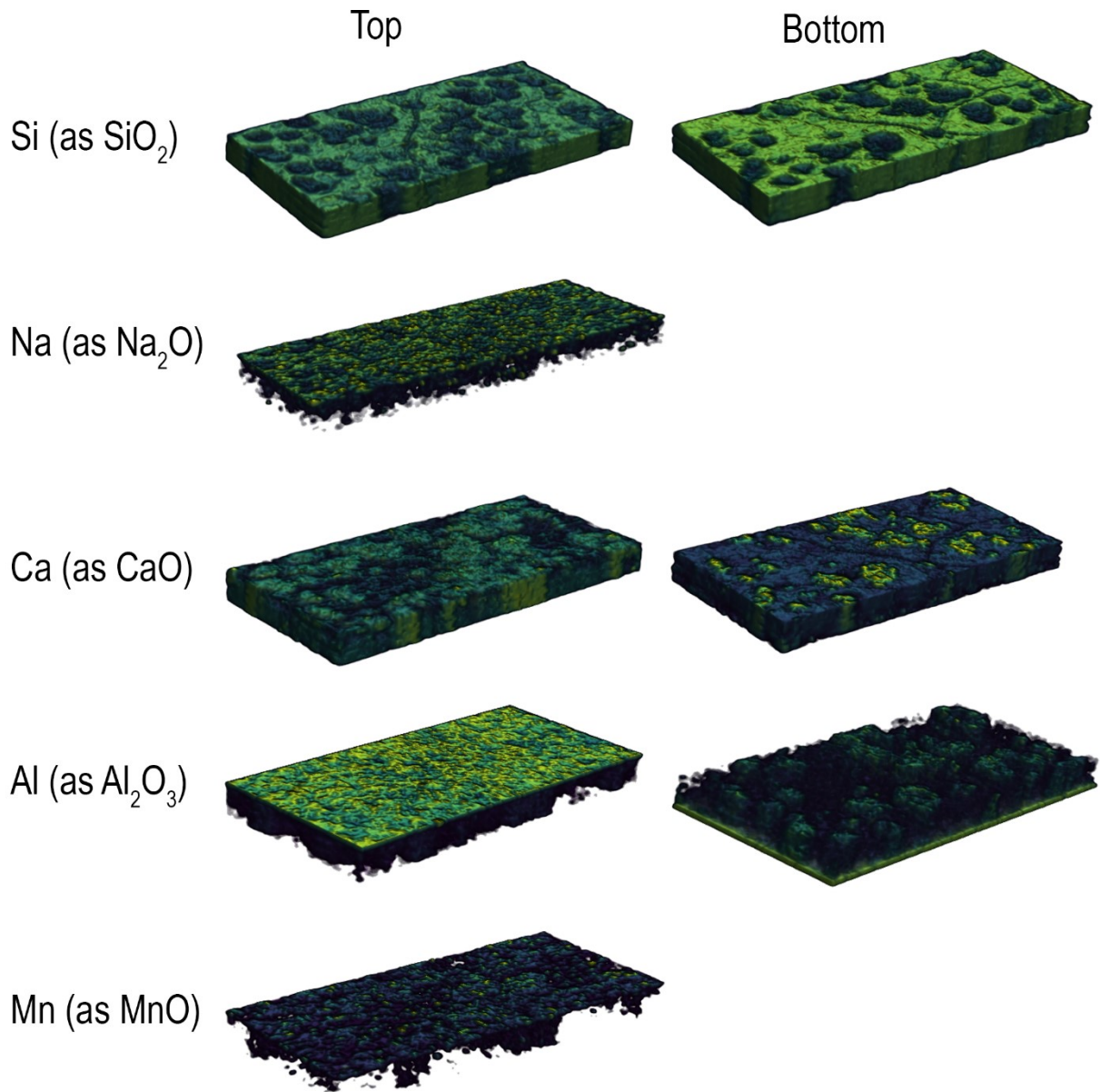
Figure S1. 3D reconstruction of the entire volume of the investigated area for each element for the pitting sample. The z axis scale is arbitrary.
