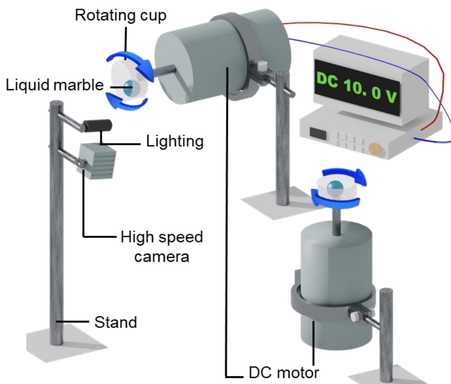
Figure S. Experimental setup to rotate the liquid marble around the horizontal axis and around the vertical axis.
