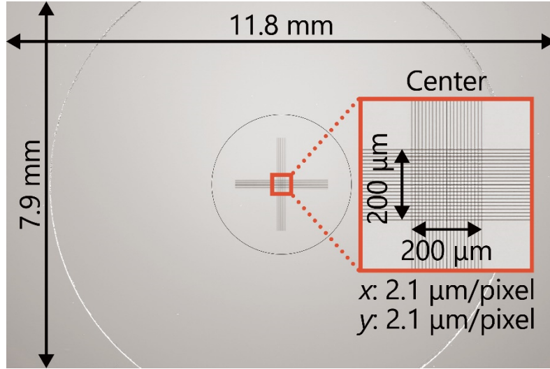
Fig. S1. Bright-field imaging with COWFISH
