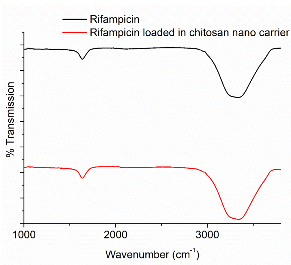
Figure S3: FT IR spectra of rifampicin and rifampicin loaded chitosan nano carriers showing no interaction with the excipients.
