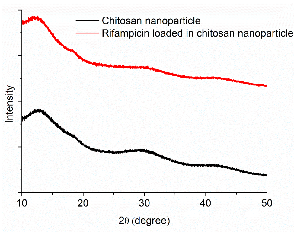
Figure S1: XRD patterns of chitosan nanoparticle and rifampicin loaded nanoparticle
