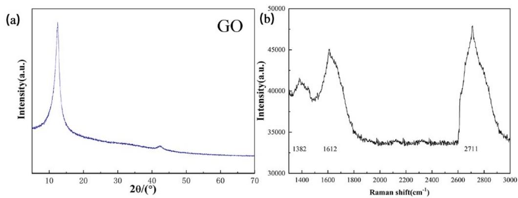
Fig. S1. XRD pattern (a) and Raman spectrum (b) of GO.
