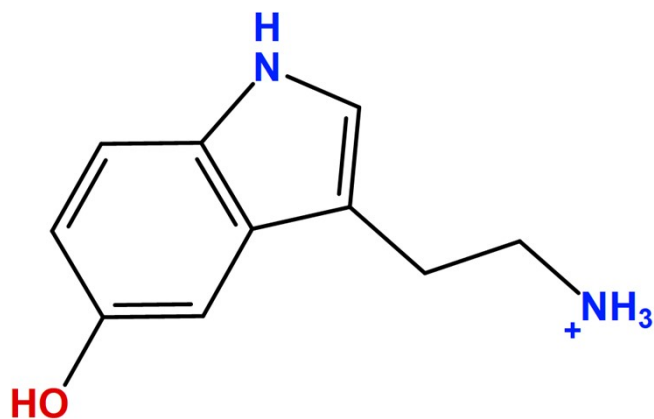
Figure S1. Structure of Serotonin after washing in MOE at pH 7
