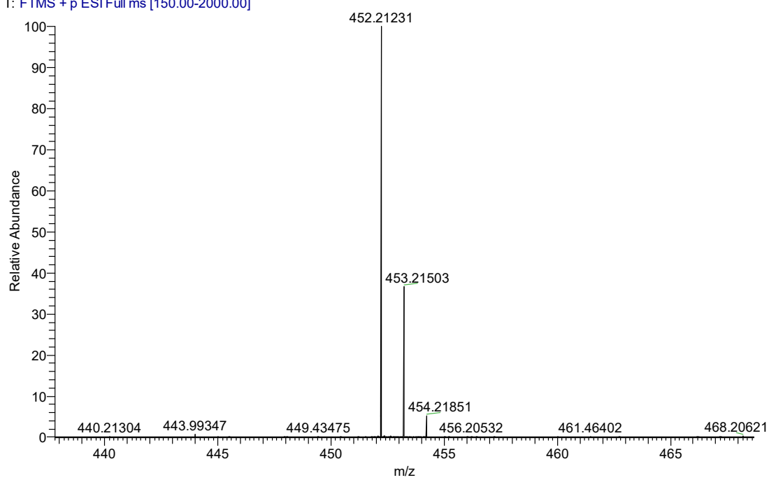
Figure S28-2 the HRMS data of compound 3ab
