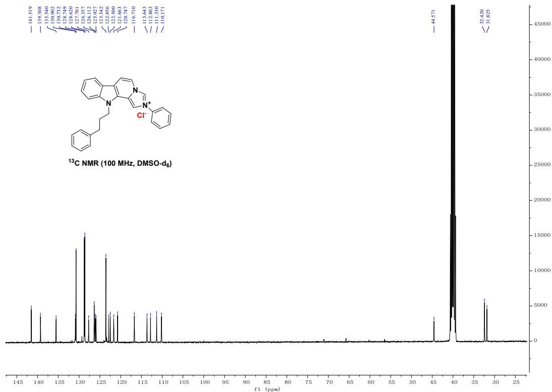
Figure S8-1 the 1 H NMR spectrum and 13 C NMR spectrum of compound 3h
