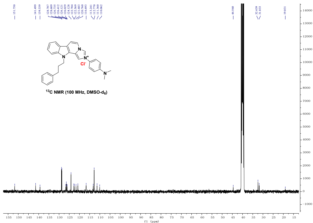
Figure S23-1 the 1 H NMR spectrum and 13 C NMR spectrum of compound 3w
