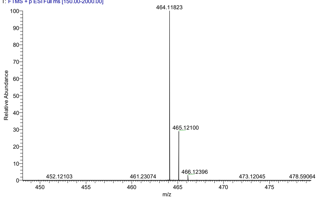
Figure S7-2 the HRMS data of compound 3g
