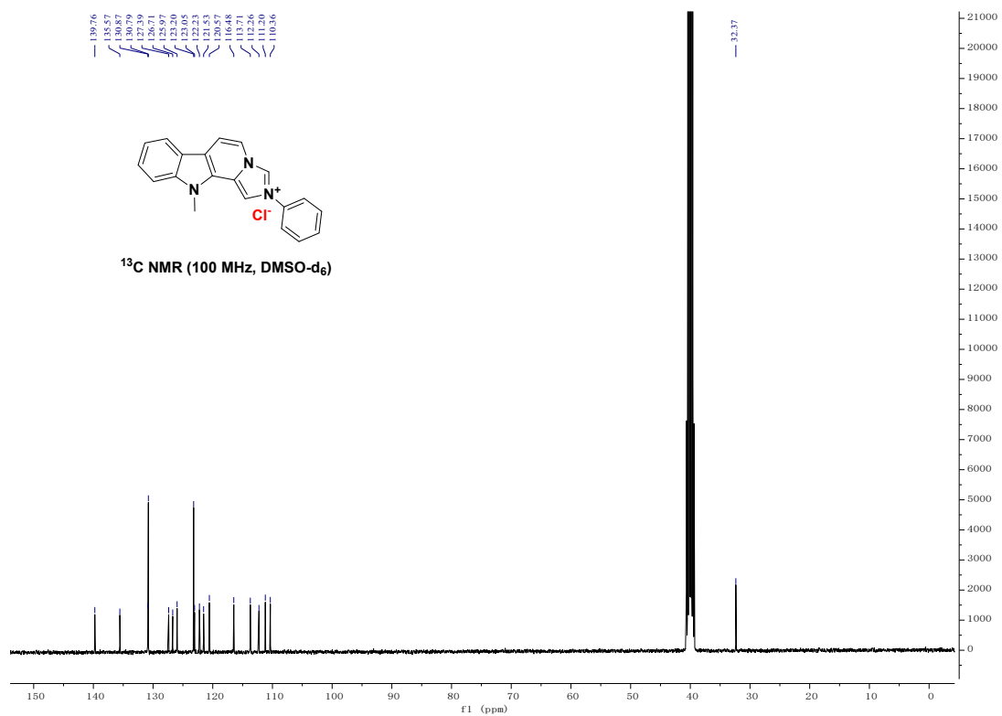
Figure S1-1 the 1 H NMR spectrum and 13 C NMR spectrum of compound 3a
