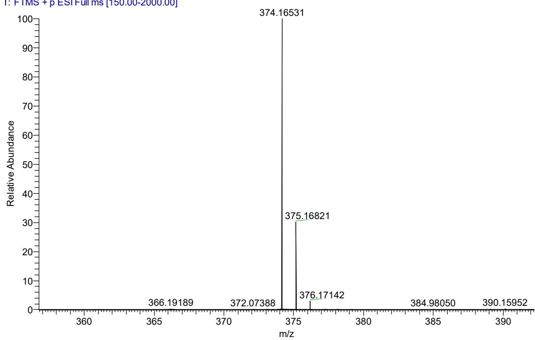
Figure S4-2 the HRMS data of compound 3d
