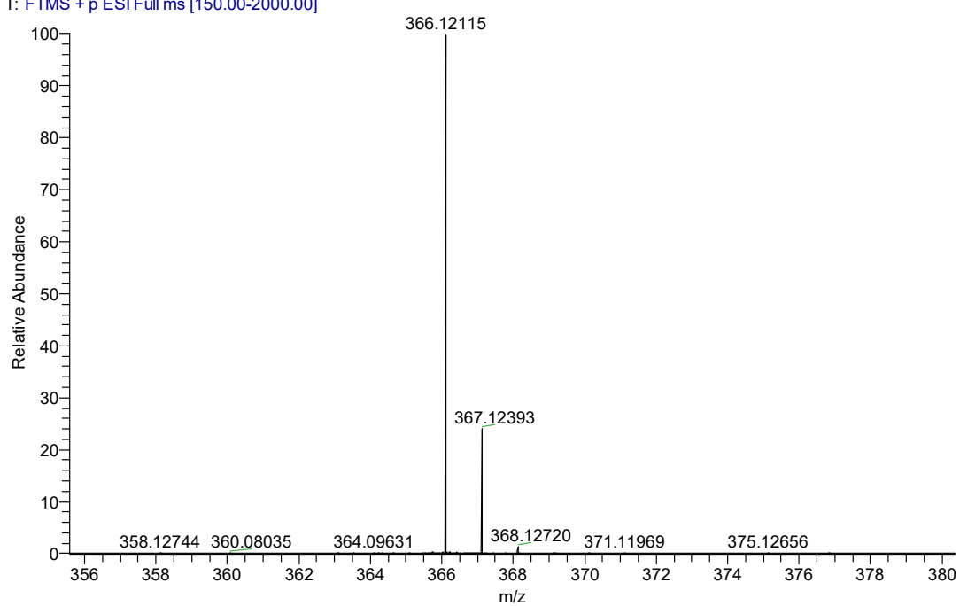
Figure S20-2 the HRMS data of compound 3t
