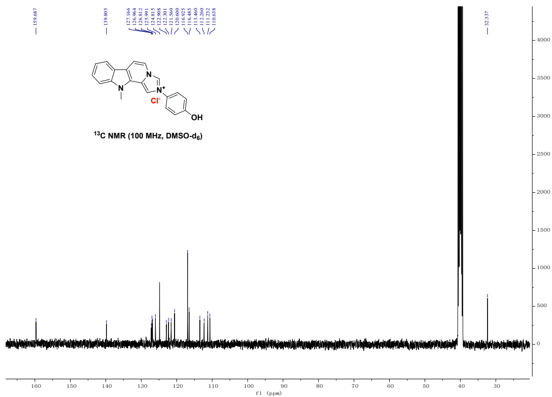
Figure S19-1 the 1 H NMR spectrum and 13 C NMR spectrum of compound 3s
