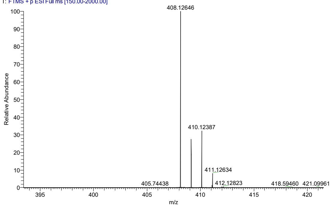
Figure S5-2 the HRMS data of compound 3e
