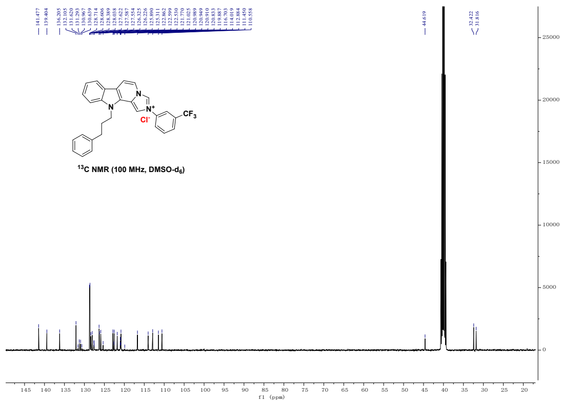
Figure S25-1 the 1 H NMR spectrum and 13 C NMR spectrum of compound 3y
