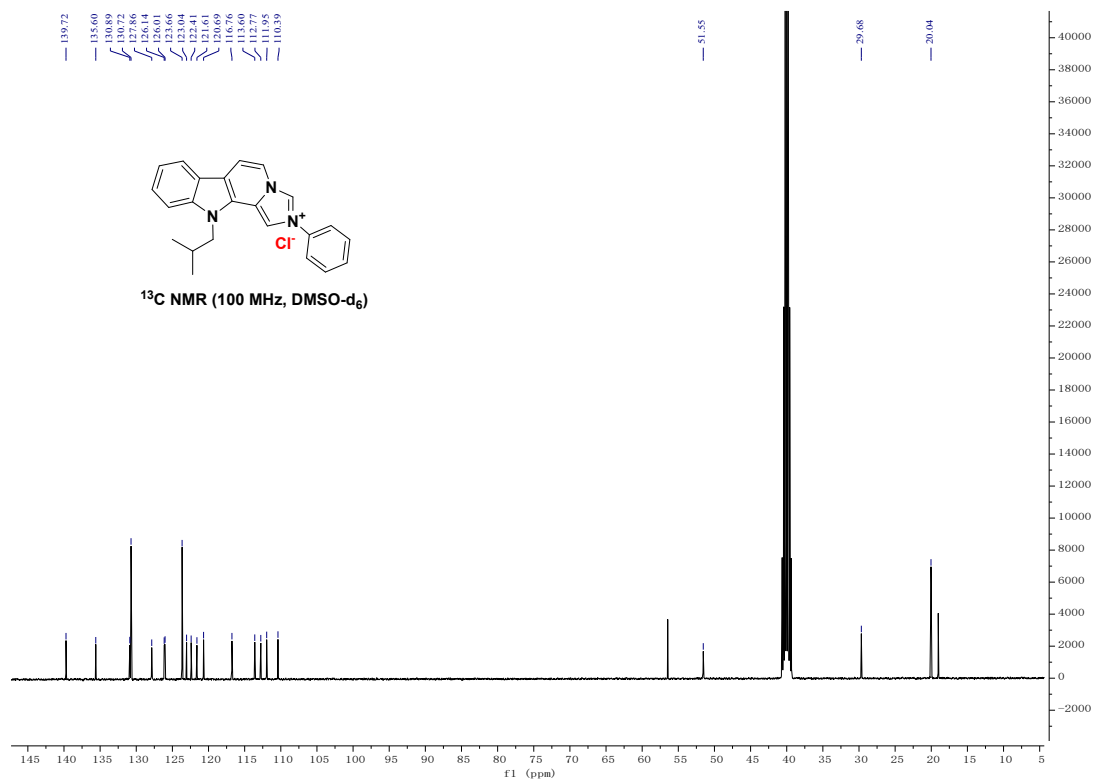
Figure S3-1 the 1 H NMR spectrum and 13 C NMR spectrum of compound 3c
