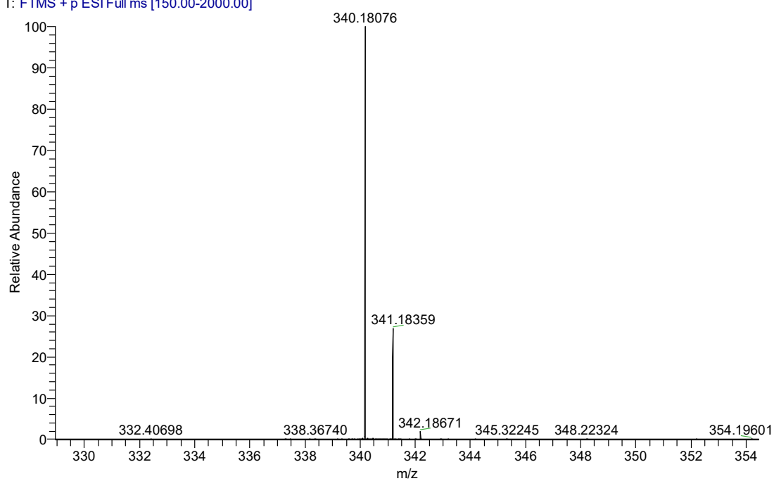
Figure S3-2 the HRMS data of compound 3c
