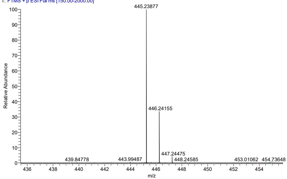
Figure S23-2 the HRMS data of compound 3w
