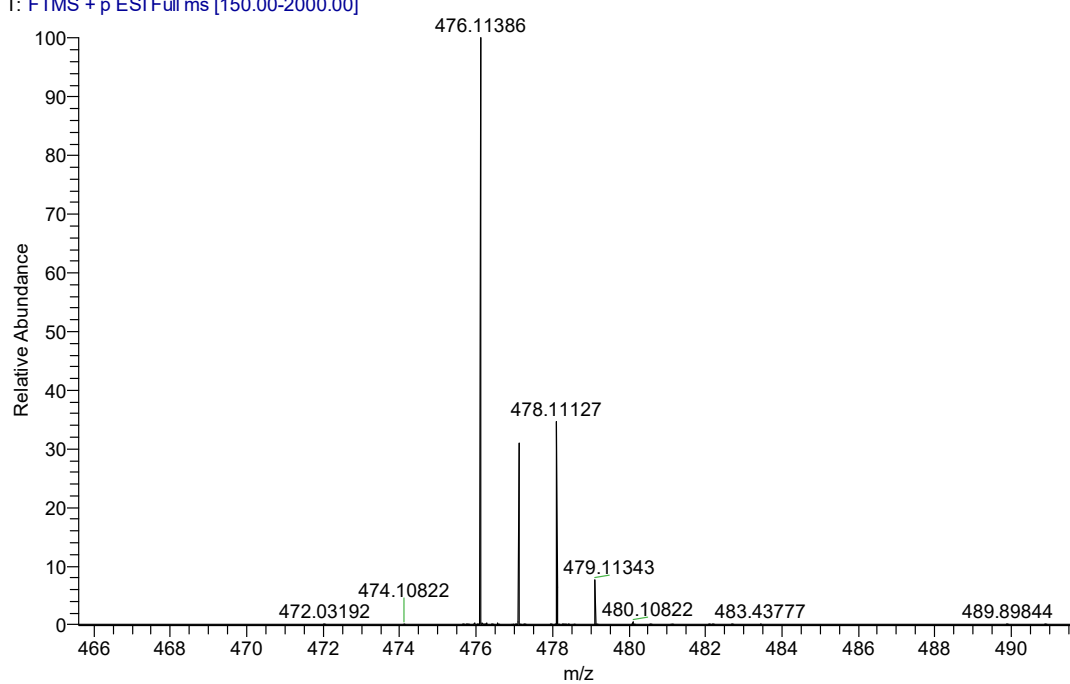
Figure S13-2 the HRMS data of compound 3m
