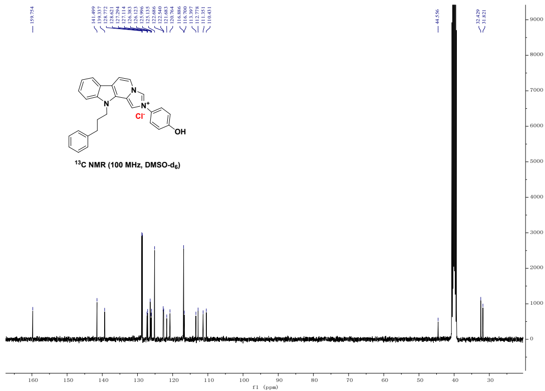
Figure S24-1 the 1 H NMR spectrum and 13 C NMR spectrum of compound 3x
