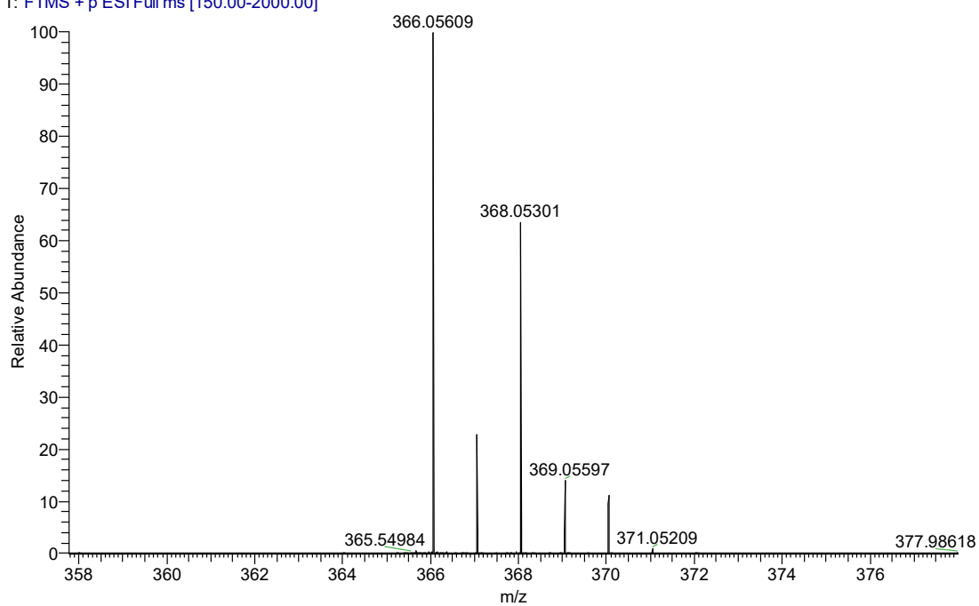
Figure S17-2 the HRMS data of compound 3q
