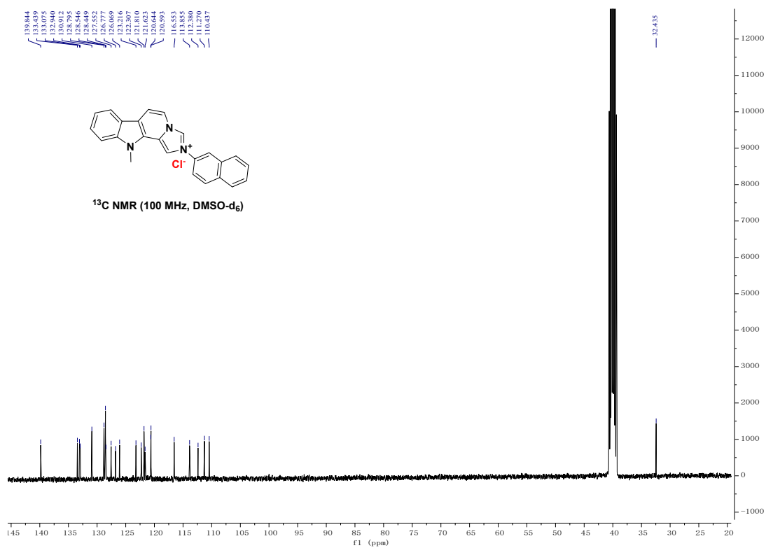
Figure S27-1 the 1 H NMR spectrum and 13 C NMR spectrum of compound 3aa
