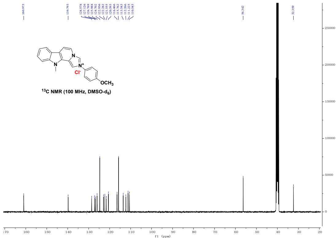
Figure S21-1 the 1 H NMR spectrum and 13 C NMR spectrum of compound 3u
