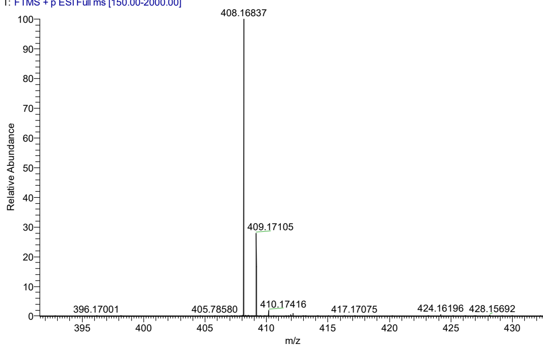
Figure S11-2 the HRMS data of compound 3k
