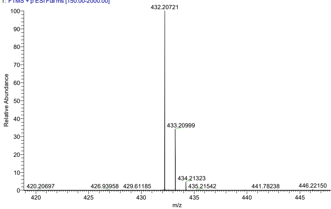
Figure S26-2 the HRMS data of compound 3z
