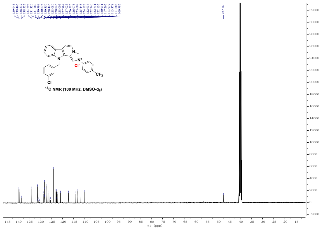
Figure S13-1 the 1 H NMR spectrum and 13 C NMR spectrum of compound 3m
