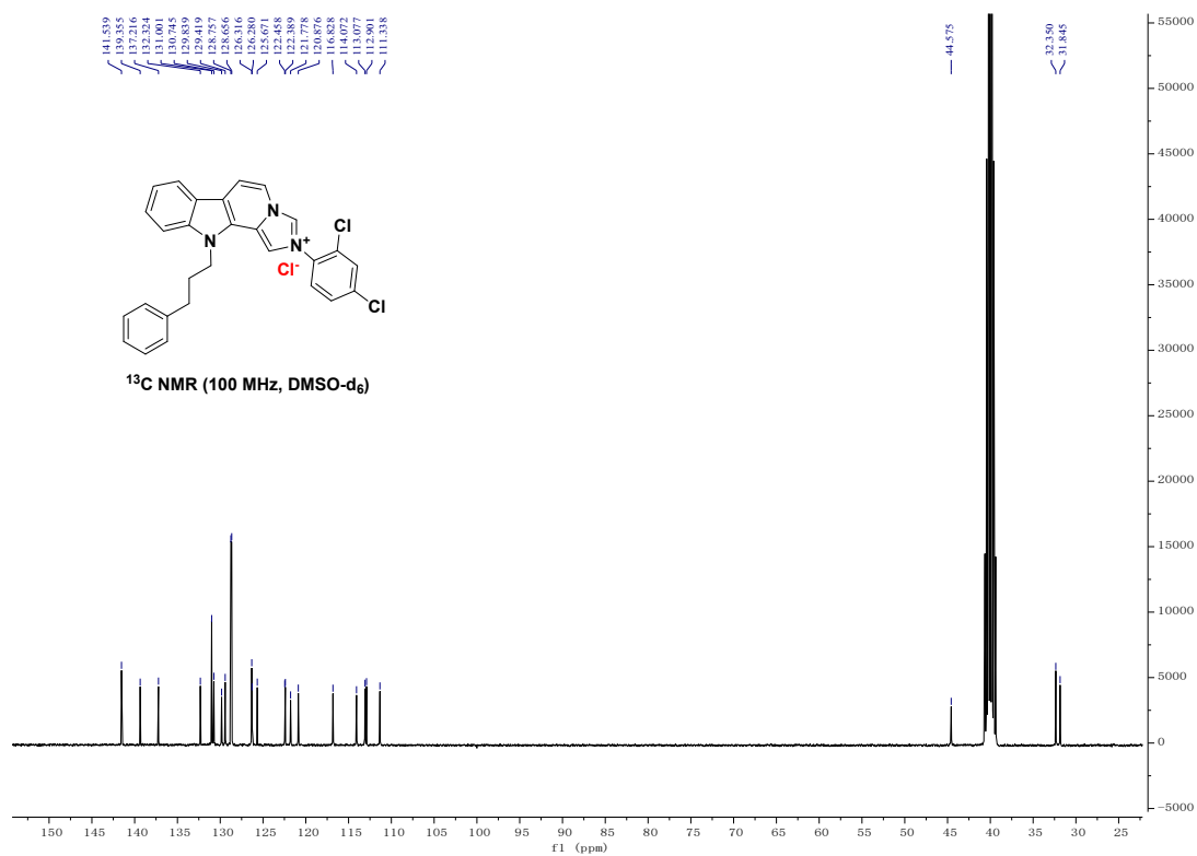
Figure S22-1 the 1 H NMR spectrum and 13 C NMR spectrum of compound 3v
