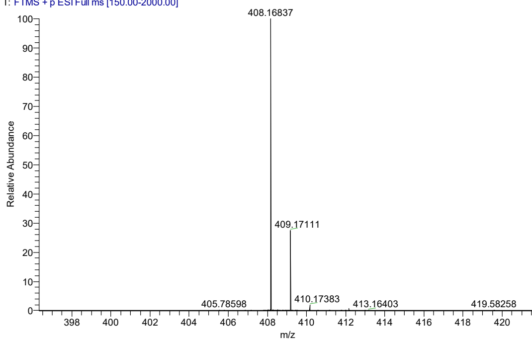
Figure S10-2 the HRMS data of compound 3j
