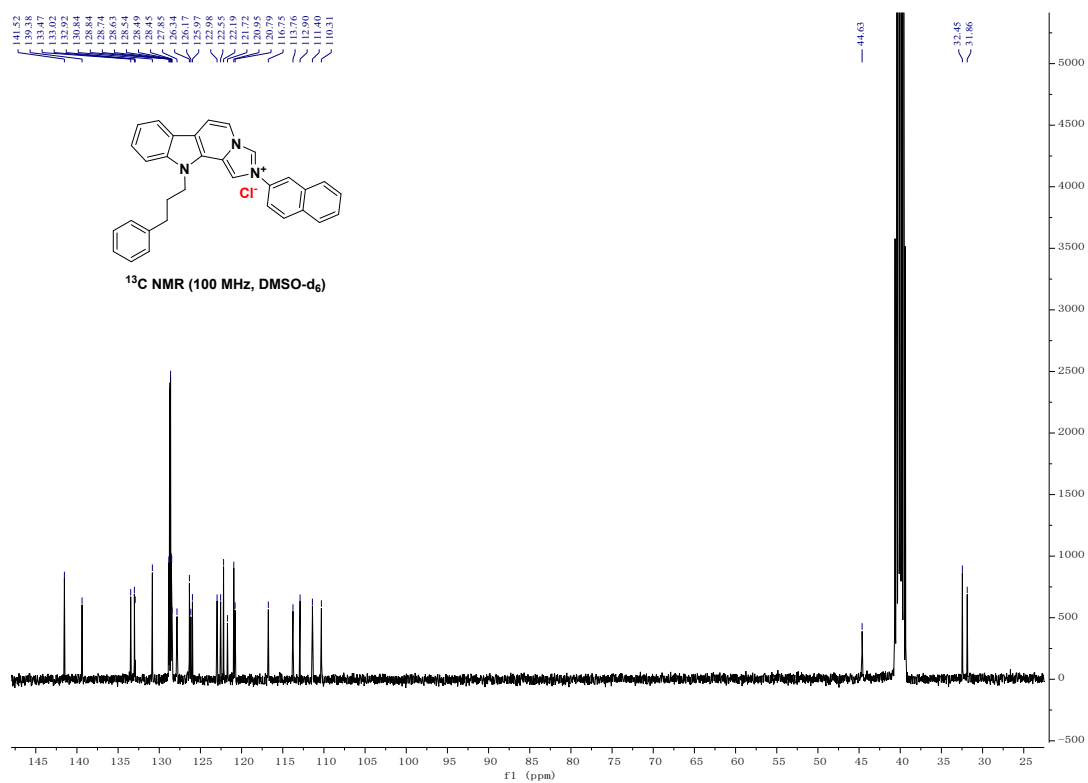
Figure S28-1 the 1 H NMR spectrum and 13 C NMR spectrum of compound 3ab
