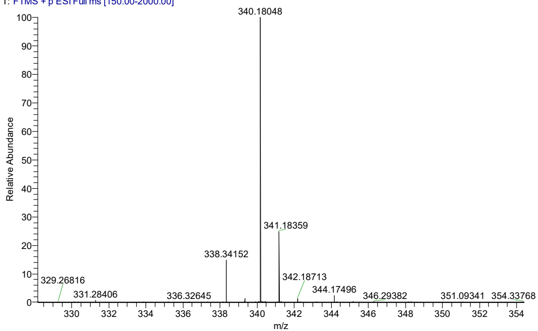
Figure S2-2 the HRMS data of compound 3b
