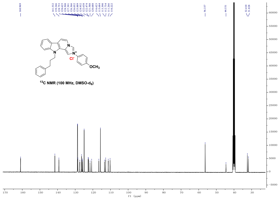
Figure S26-1 the 1 H NMR spectrum and 13 C NMR spectrum of compound 3z
