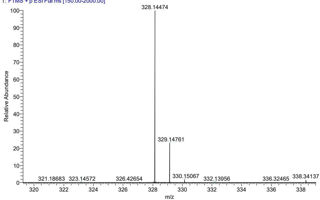
Figure S21-2 the HRMS data of compound 3u
