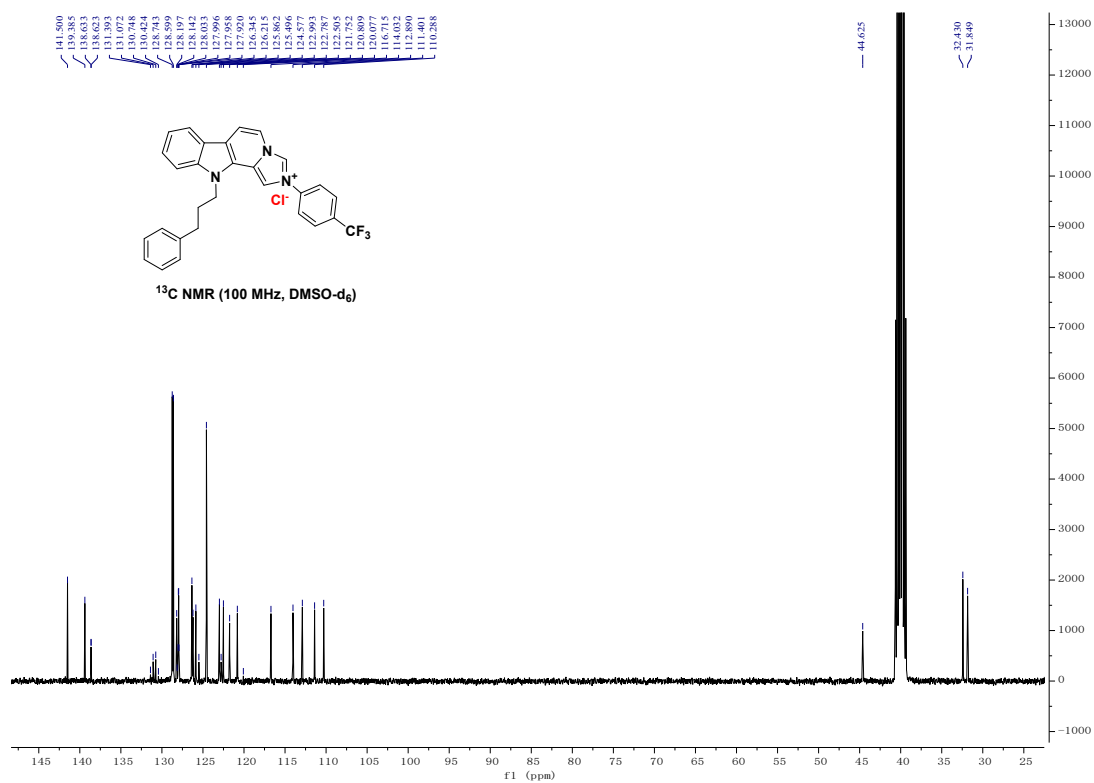
Figure S16-1 the 1 H NMR spectrum and 13 C NMR spectrum of compound 3p
