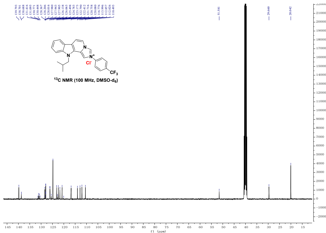
Figure S11-1 the 1 H NMR spectrum and 13 C NMR spectrum of compound 3k
