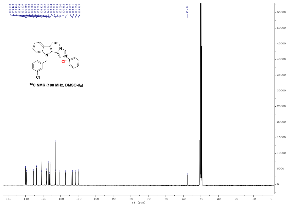
Figure S5-1 the ^1\text{H} NMR spectrum and ^{13}\text{C} NMR spectrum of compound 3e
