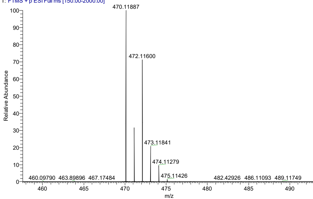
Figure S22-2 the HRMS data of compound 3v
