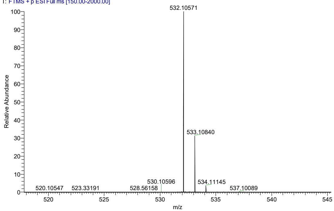
Figure S15-2 the HRMS data of compound 3o
