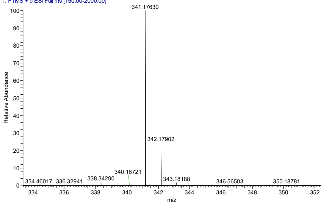
Figure S18-2 the HRMS data of compound 3r
