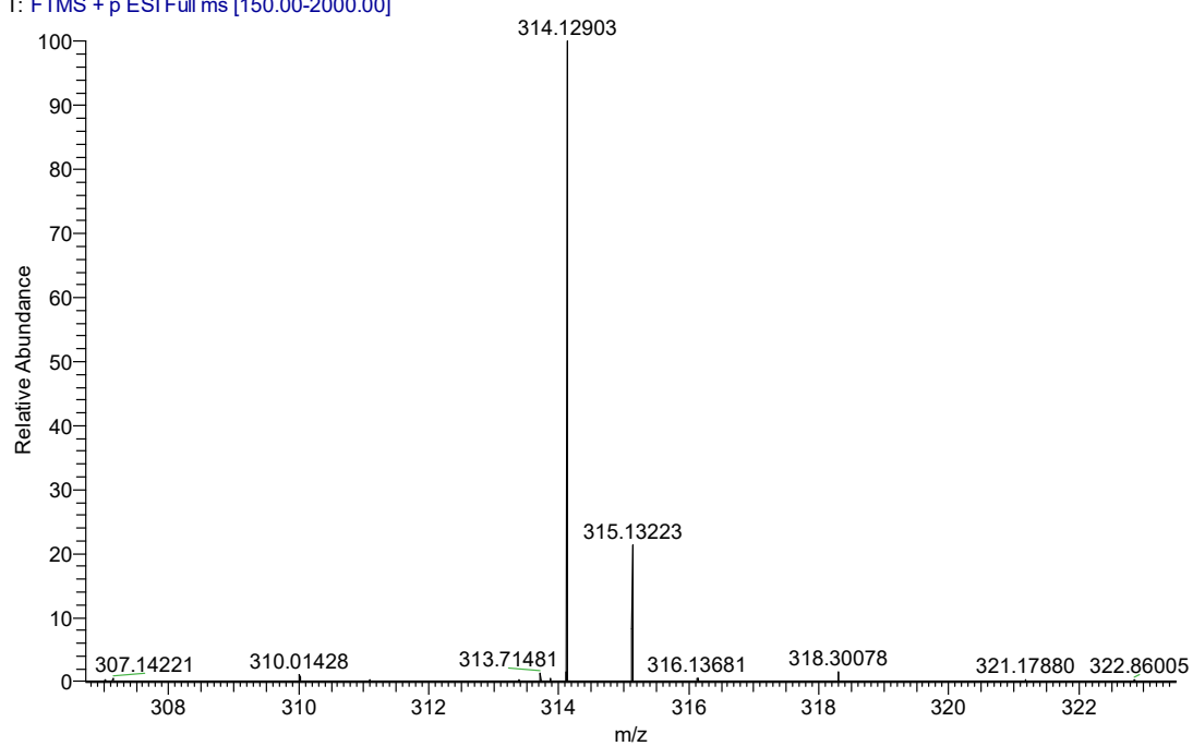
Figure S19-2 the HRMS data of compound 3s
