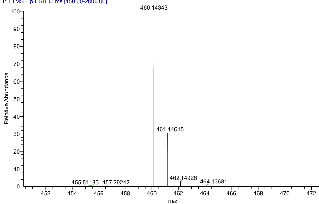
Figure S14-2 the HRMS data of compound 3n
