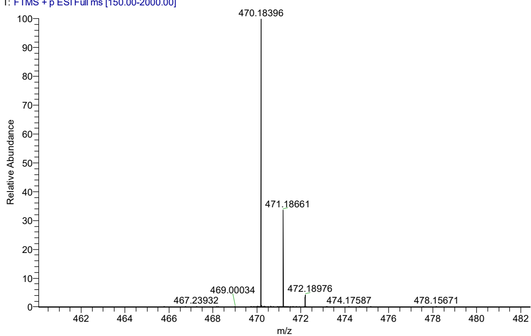
Figure S25-2 the HRMS data of compound 3y
