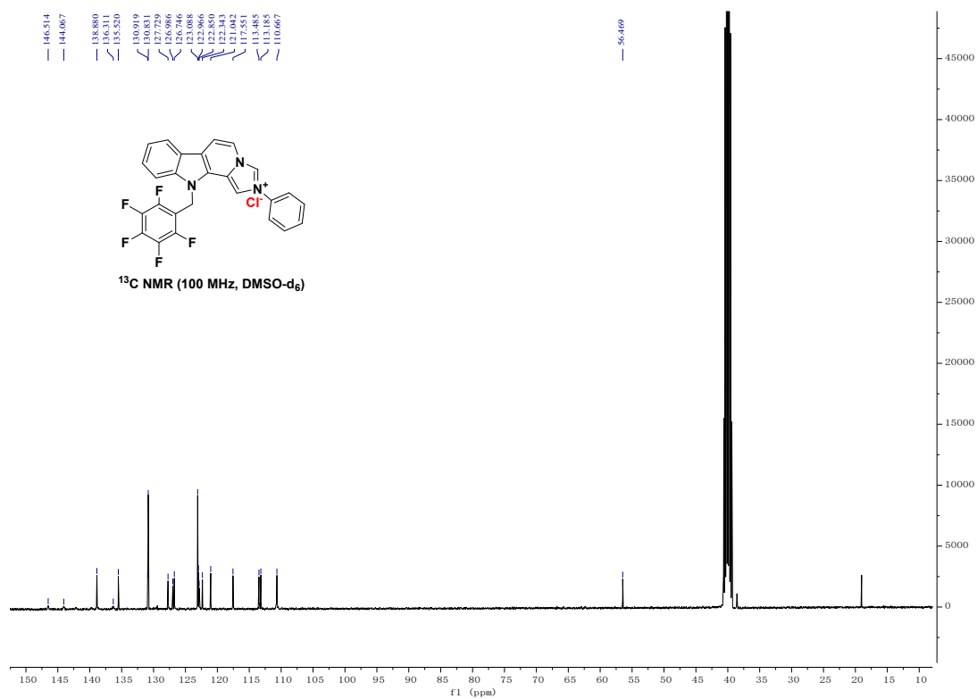
Figure S7-1 the 1 H NMR spectrum and 13 C NMR spectrum of compound 3g
