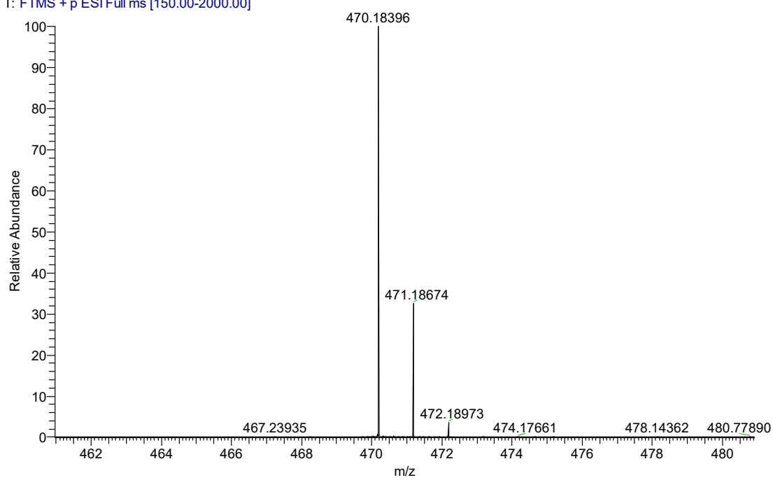
Figure S16-2 the HRMS data of compound 3p
