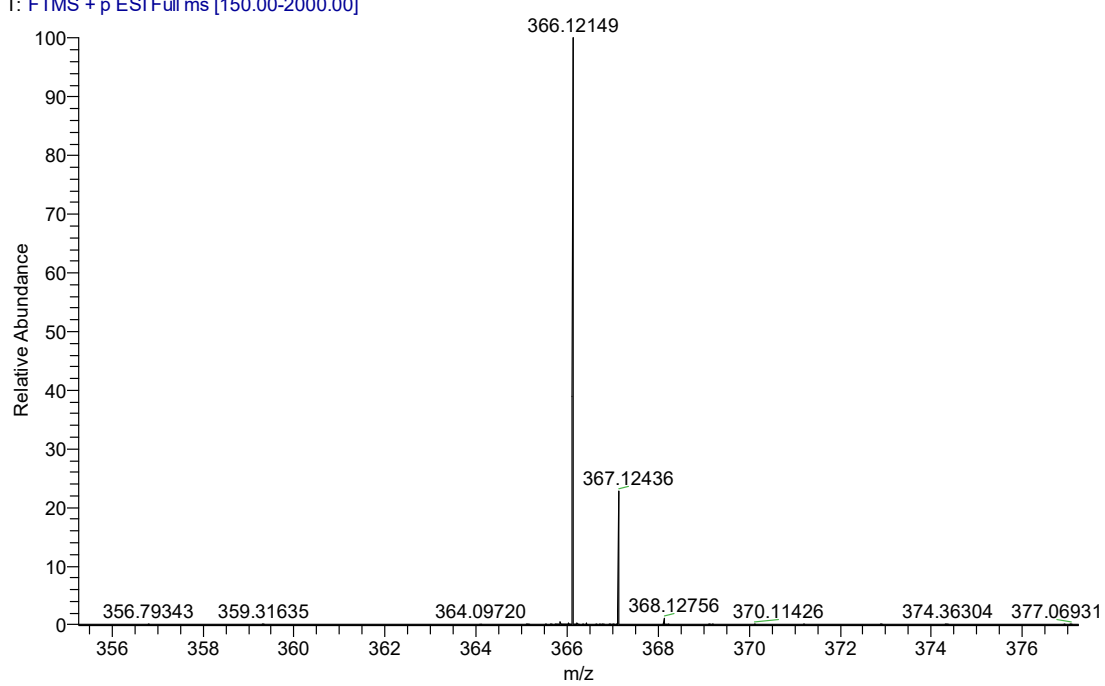
Figure S9-2 the HRMS data of compound 3i
