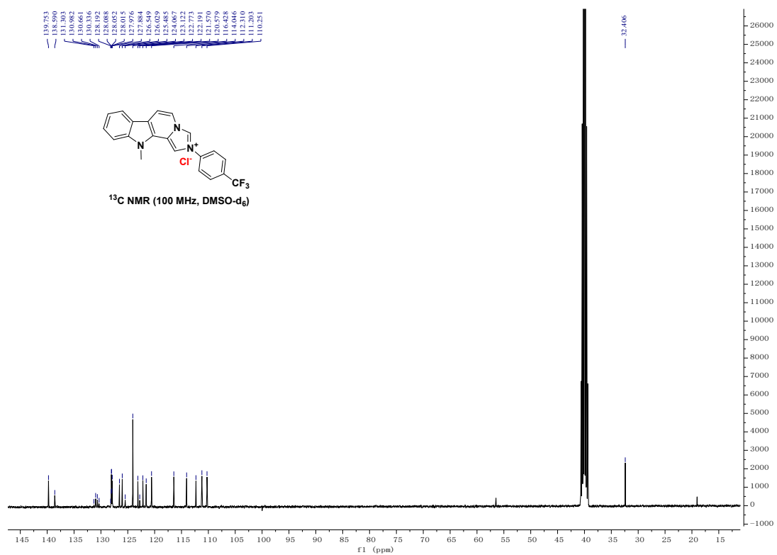
Figure S9-1 the 1 H NMR spectrum and 13 C NMR spectrum of compound 3i
