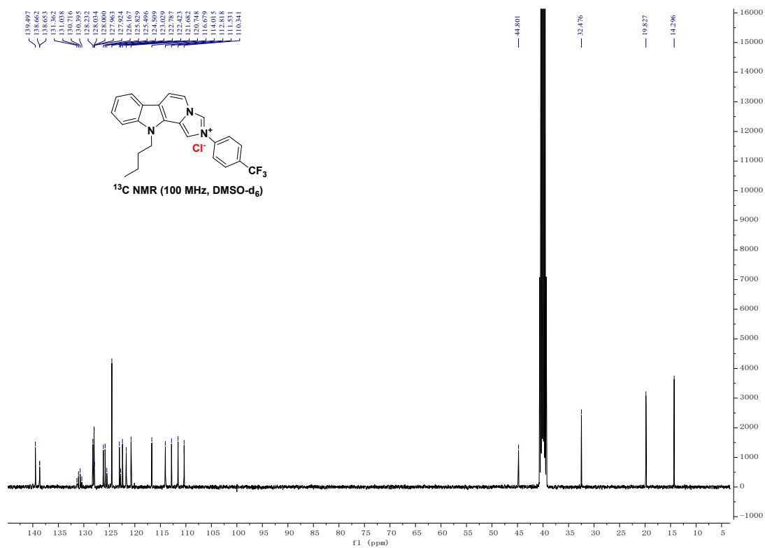
Figure S10-1 the 1 H NMR spectrum and 13 C NMR spectrum of compound 3j
