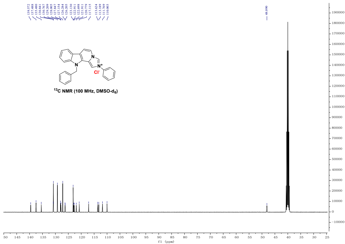
Figure S4-1 the 1 H NMR spectrum and 13 C NMR spectrum of compound 3d
