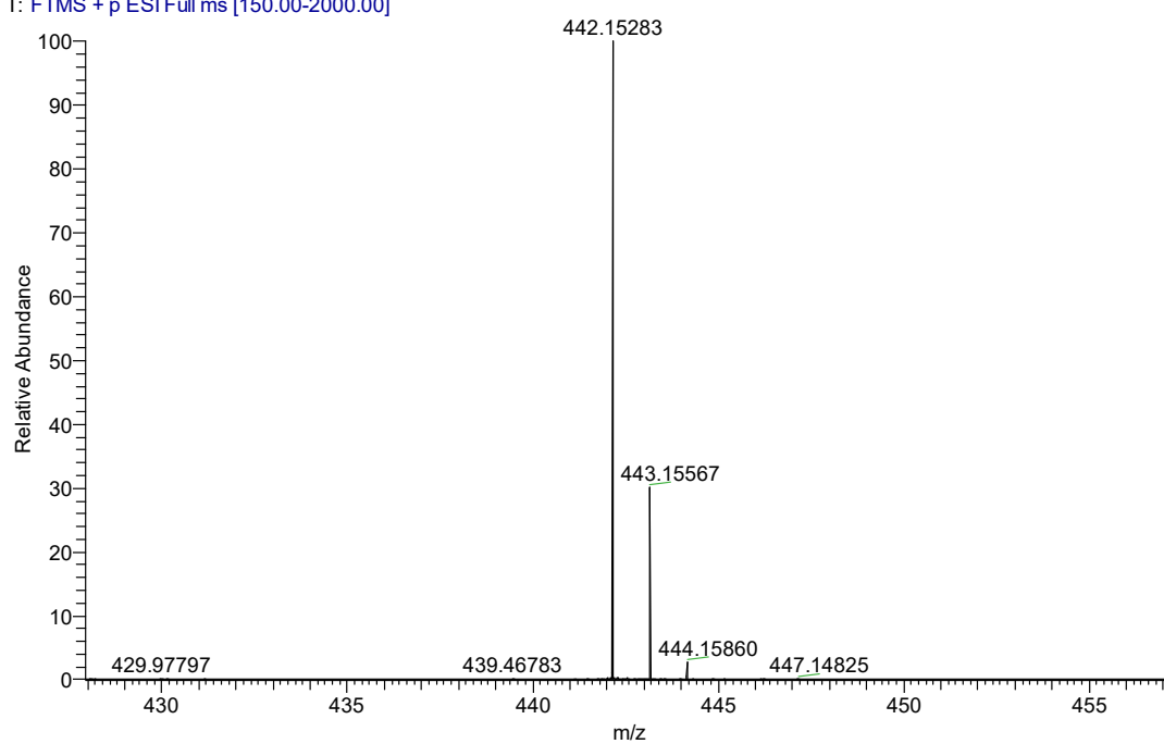
Figure S12-2 the HRMS data of compound 31
