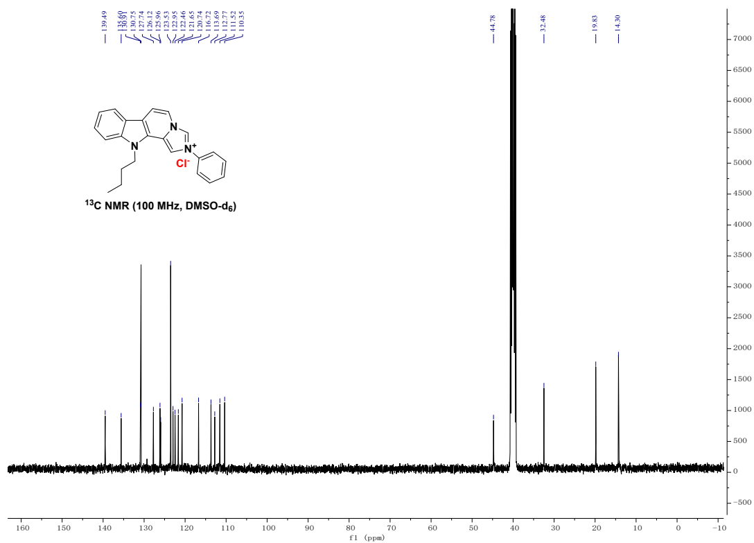
Figure S2-1 the 1 H NMR spectrum and 13 C NMR spectrum of compound 3b
