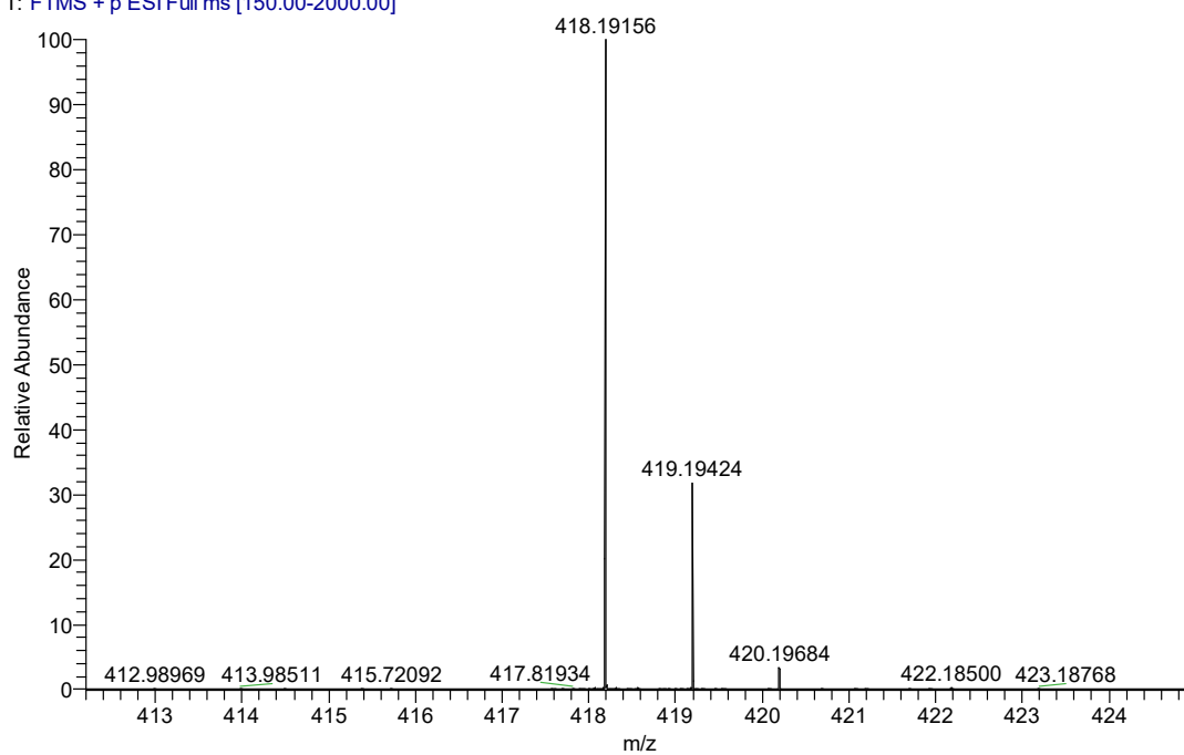
Figure S24-2 the HRMS data of compound 3x
