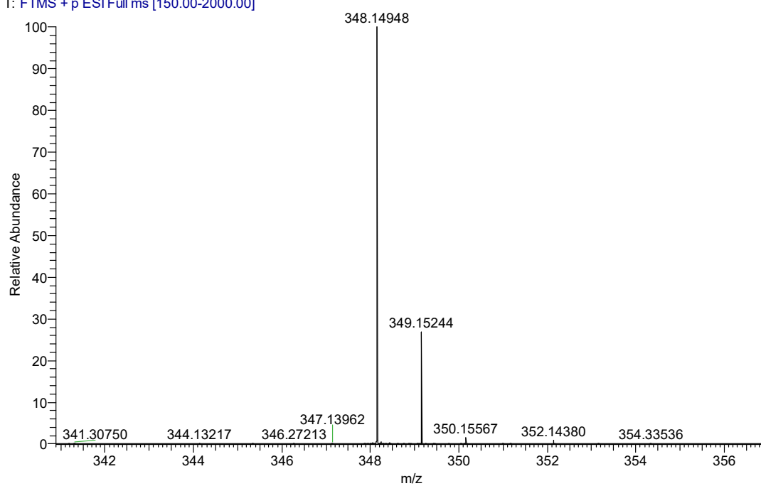
Figure S27-2 the HRMS data of compound 3aa
