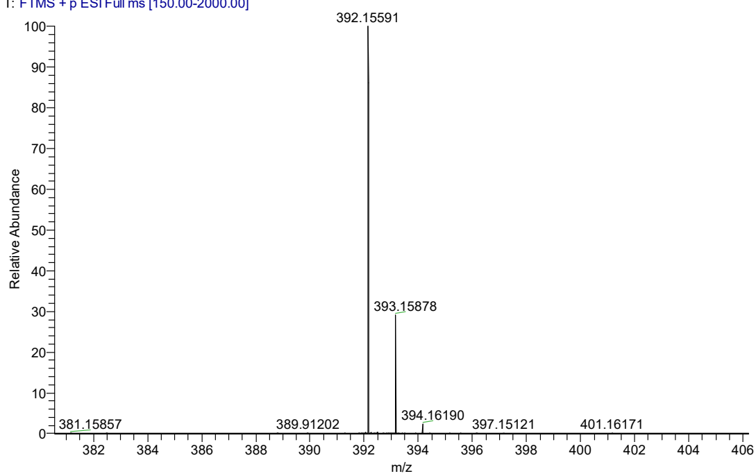
Figure S6-2 the HRMS data of compound 3f
