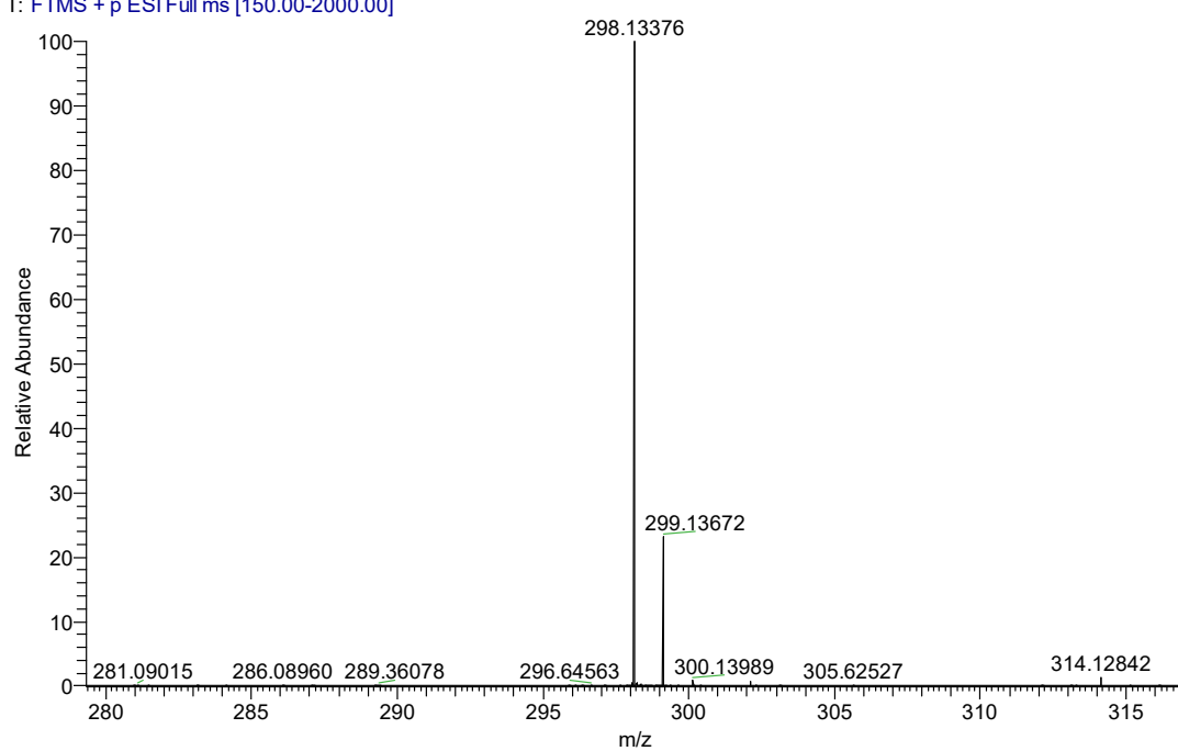
Figure S1-2 the HRMS data of compound 3a
