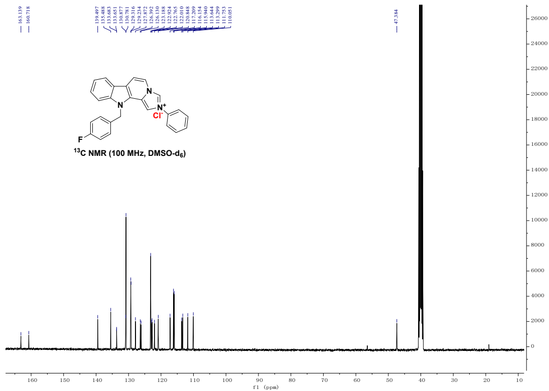
Figure S6-1 the 1 H NMR spectrum and 13 C NMR spectrum of compound 3f
