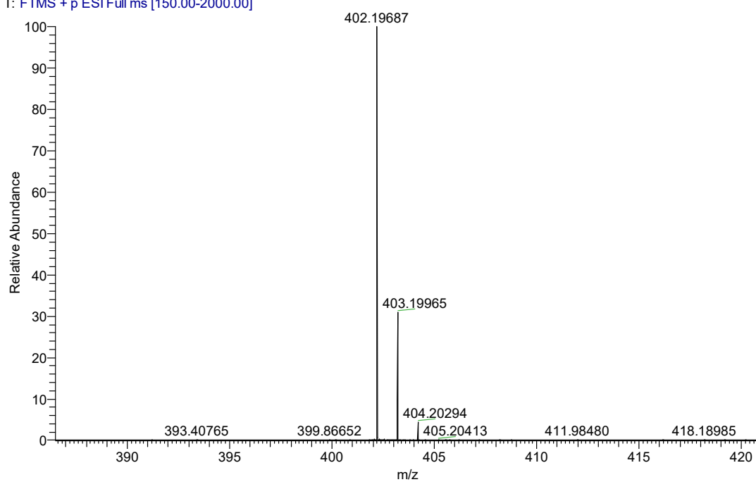
Figure S8-2 the HRMS data of compound 3h
