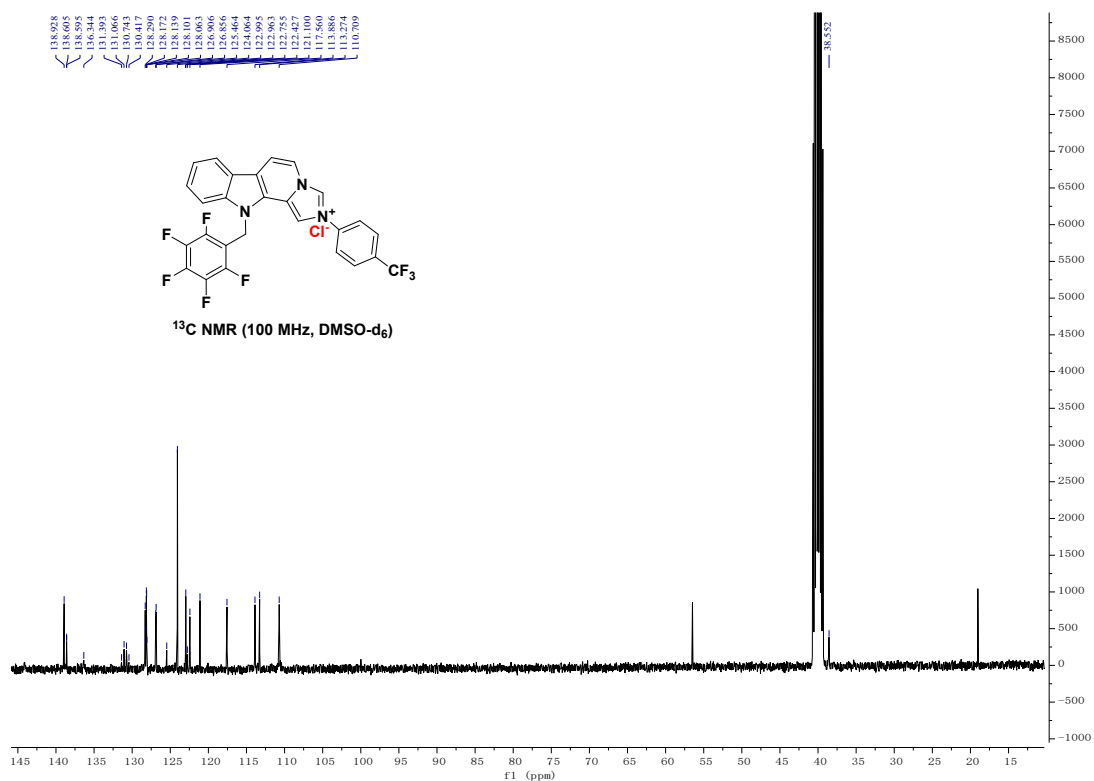
Figure S15-1 the 1 H NMR spectrum and 13 C NMR spectrum of compound 30
