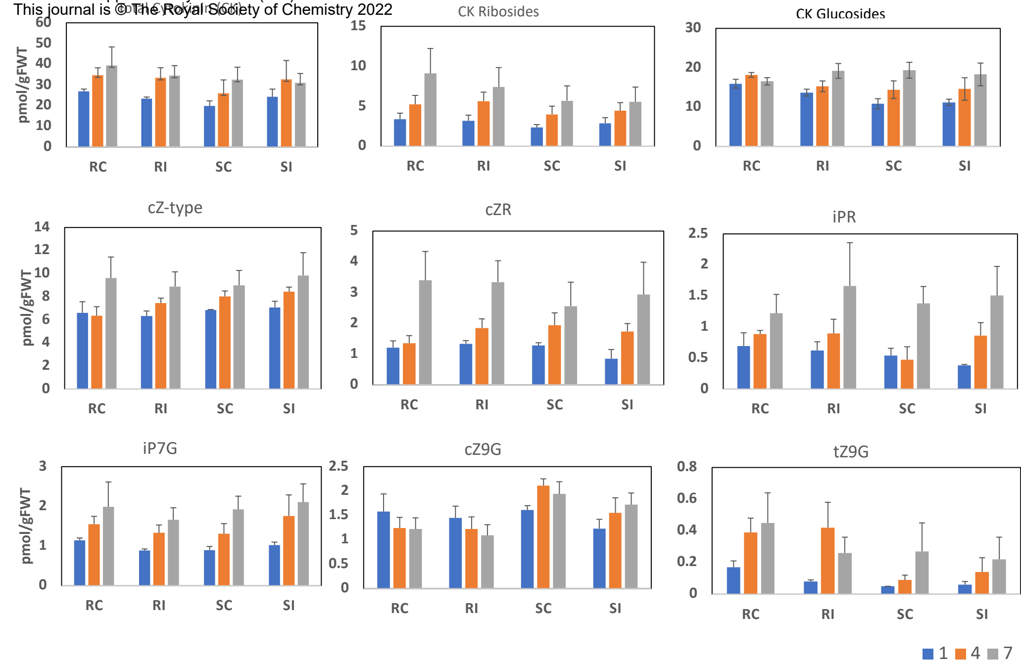
Fig. S6 Endogenous cytokinin concentration in root tissues. Error bar indicates the standard errors of mean (n=3). 1-, 4-, and 7- DPI= indicates, days post inoculation (DPI); RC=Resistant uninoculated, RI=Resistant inoculated, SC=Susceptible uninoculated, SI=Susceptible inoculated.
