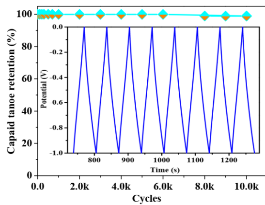
Figure S4 Cycling performance of GLAC-2 at 10 A g -1
