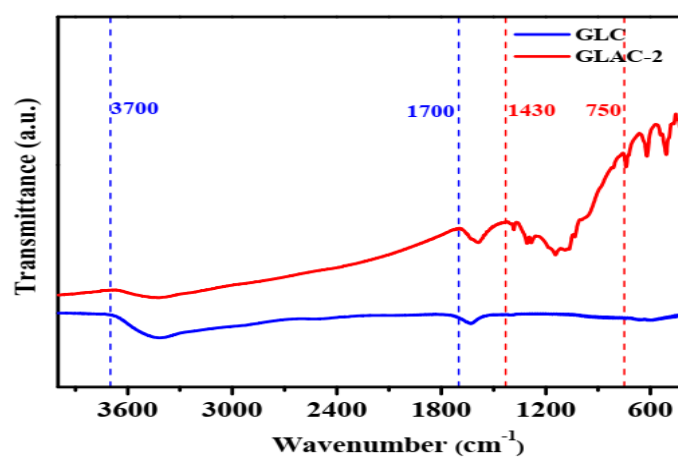
Figure S2 FTIR spectra of GLC and GLAC-2
