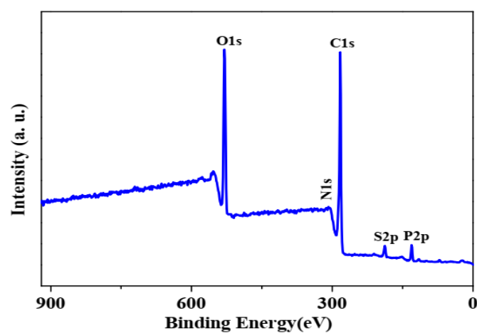
Figure S3 XPS survey spectrum of GLAC-2
