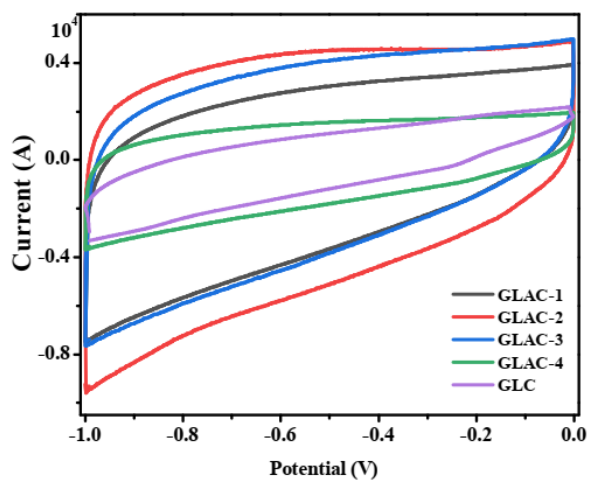
Figure S5 CV curves of GLAC samples prepared under different temperature at 100 mV/s
