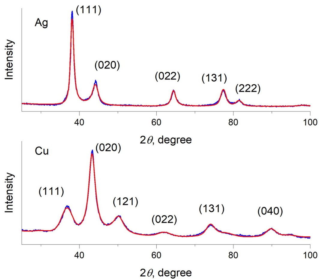
Figure S 2 XRD patterns obtained on Ag and Cu NPs. Blue curves are data, red curves are fits.
