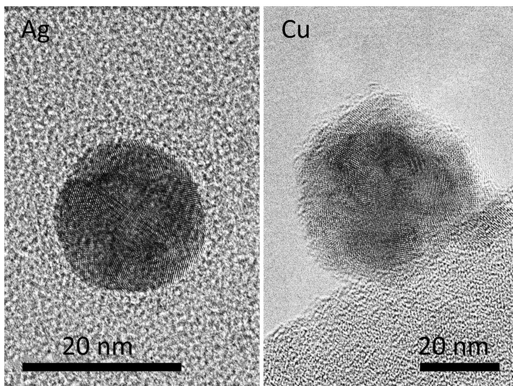
Figure S 1 High-resolution TEM images of Ag and Cu NPs prepared by dc magnetron sputtering using GAS.
