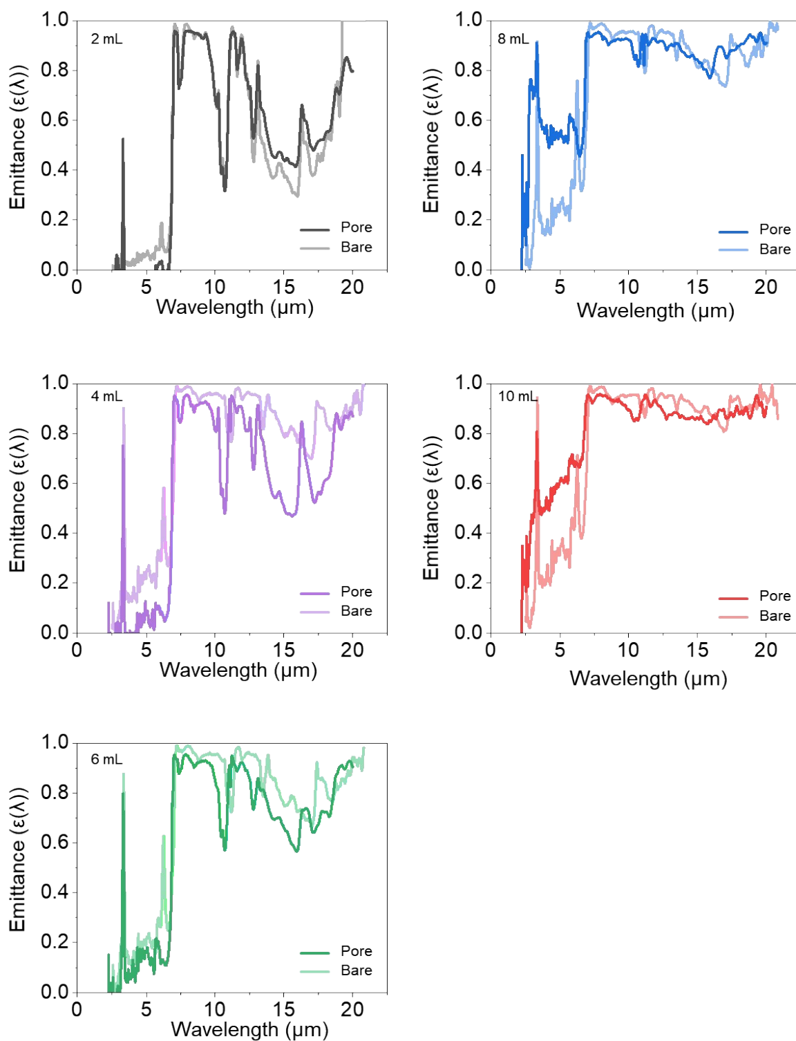
Figure S1. FTIR comparison between porous and pristine PVDF-HFP film of different thickness
