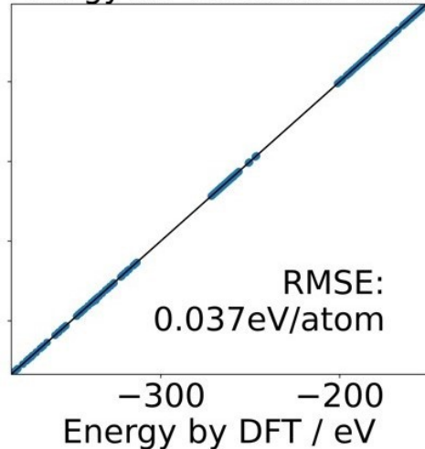
Energy on validation data
