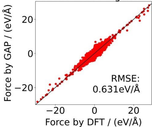
Force on training data
