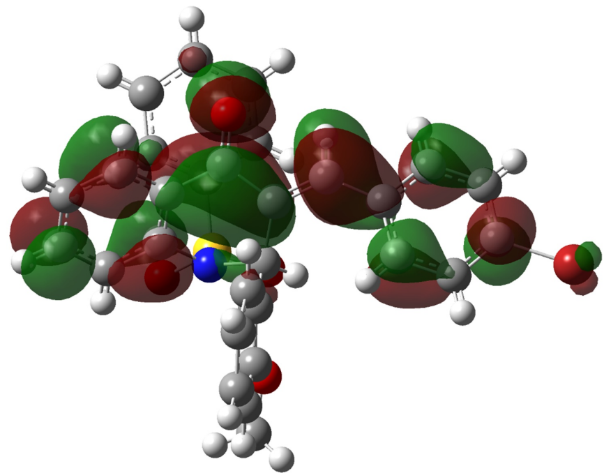
LUMO (-42.91 kcal/mol)
