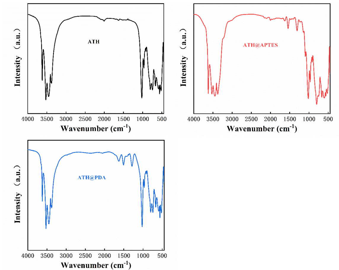
Fig. S2 FTIR spectra of ATH, ATH@APTES, ATH@PDA.
