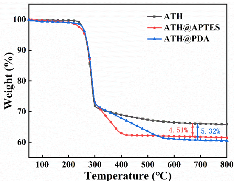
Fig. S1 The TGA curves of ATH, ATH@APTES, ATH@PDA.
