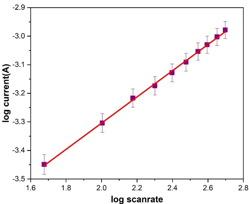
Fig S1 Plot of log scan rate vs log current.
