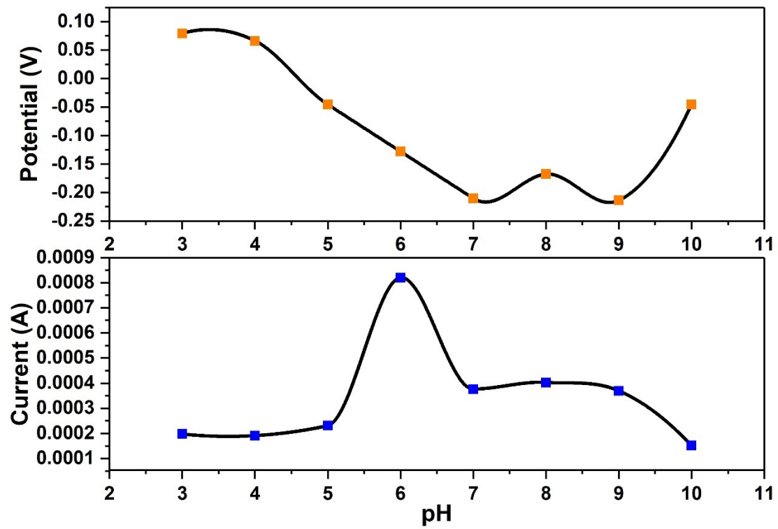
Fig S2 Plot of pH vs potential and pH vs current
